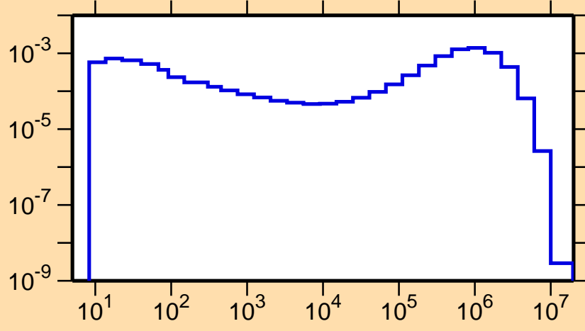
\sigma vs. E for ^{141}\text{Gd}(n,n_3)
