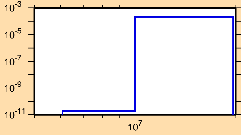
\sigma vs. E for ^{141}\text{Gd}(n,t)
