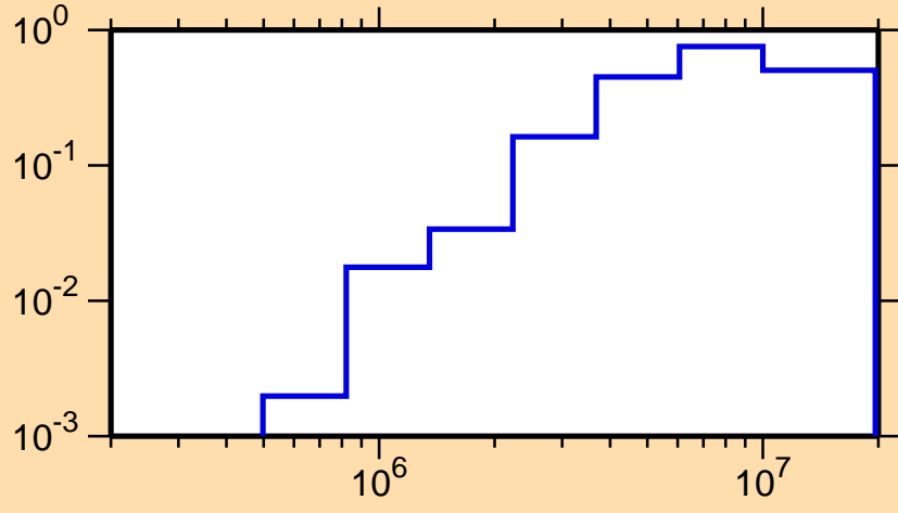
\sigma vs. E for ^{141}\text{Gd}(n,n\text{cont.})
