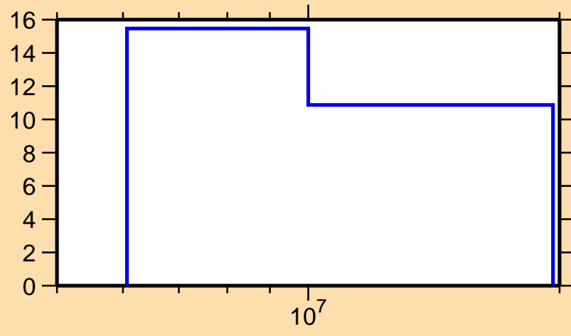
\Delta\sigma/\sigma vs. E for ^{141}\text{Gd}(n,\text{el.})
