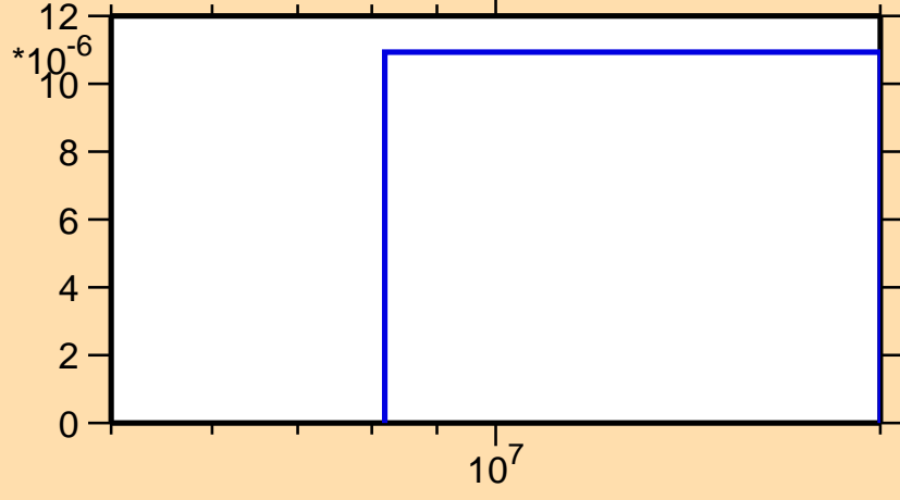
\sigma vs. E for ^{141}\text{Gd}(n,\text{pd})
