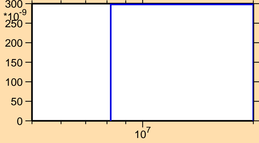
\sigma vs. E for ^{141}\text{Gd}(n,\text{pt})
