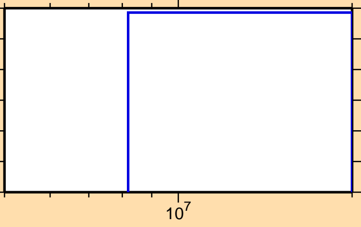
\sigma vs. E for ^{141}\text{Gd} (mt 34)
