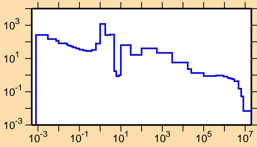
\sigma vs. E for ^{142}\text{Gd}(n,\gamma)
