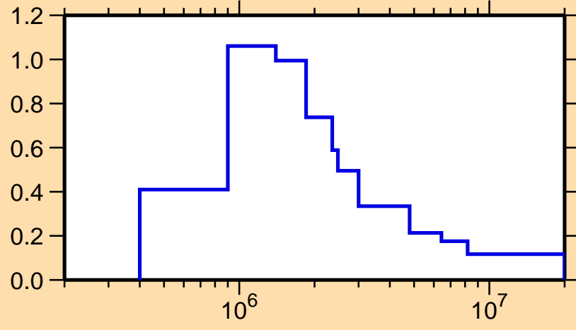
\sigma vs. E for ^{142}\text{Gd}(n,n_1)
