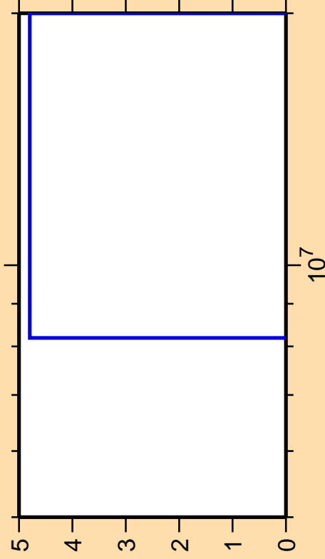
\Delta\sigma/\sigma vs. E for ^{142}\text{Gd}(\text{mt } 34)
