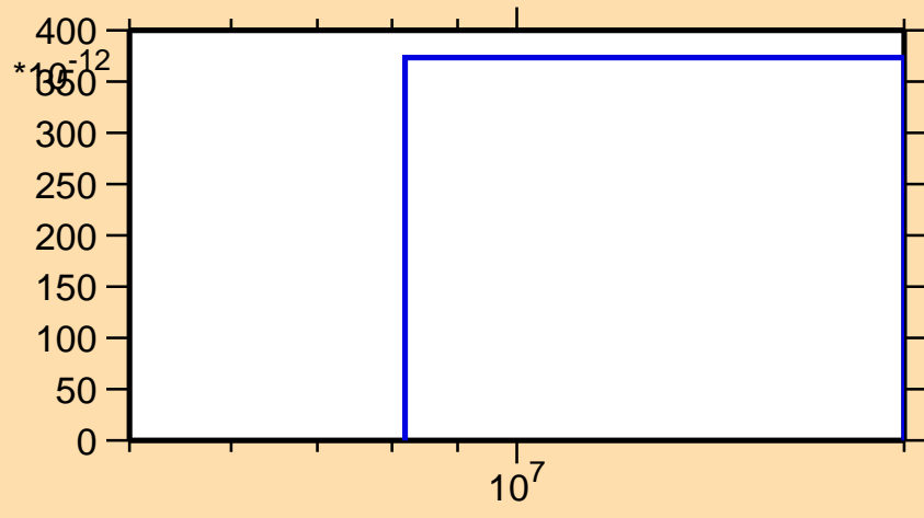
\sigma vs. E for ^{142}\text{Gd}(n,2n\alpha)
