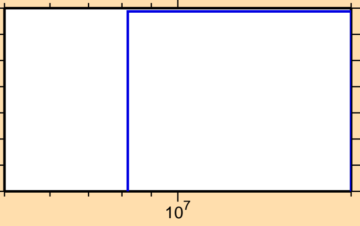
\sigma vs. E for ^{142}\text{Gd}(n,\text{pt})
