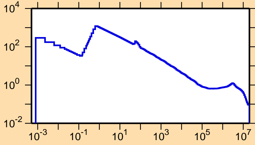
\sigma vs. E for ^{143}\text{Gd}(n,p)
