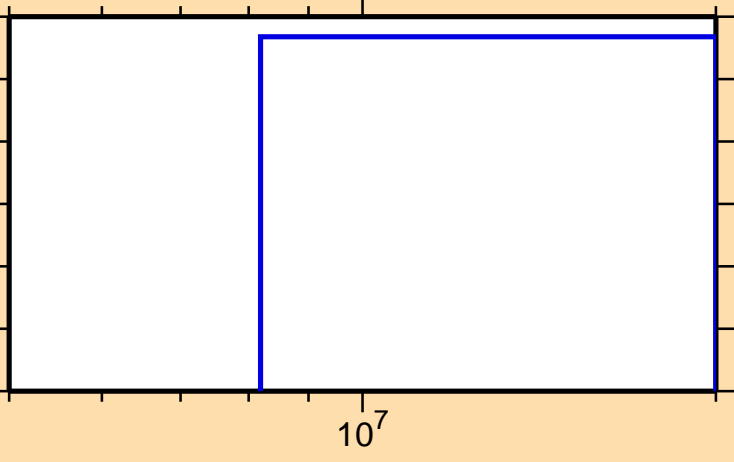
\sigma vs. E for ^{143}\text{Gd}(n,2np)
