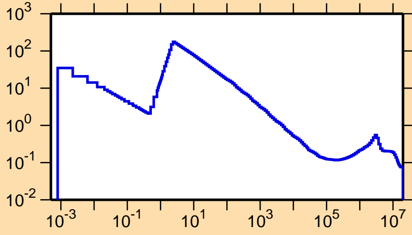
\sigma vs. E for ^{145}\text{Gd}(n,p)
