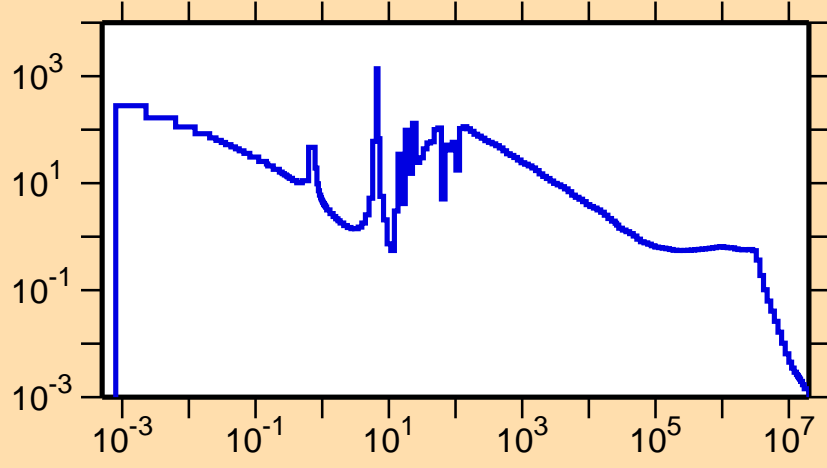
\sigma vs. E for ^{145}\text{Gd}(n,\gamma)
