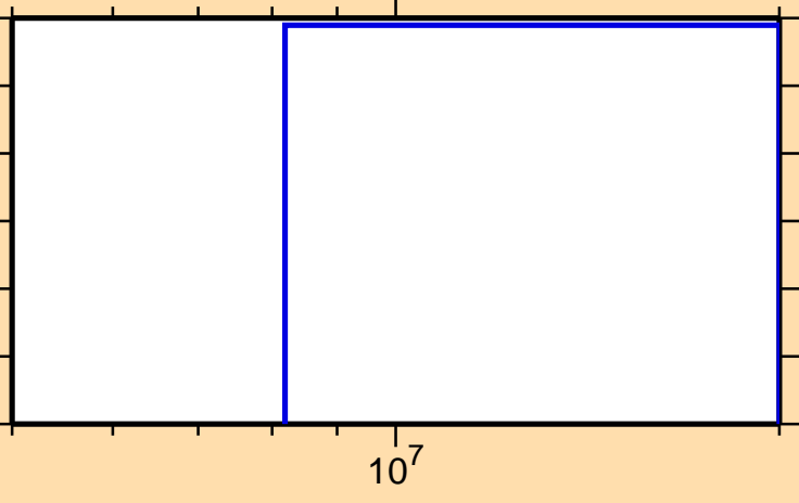
\sigma vs. E for ^{145}\text{Gd}(n,\text{nd})
