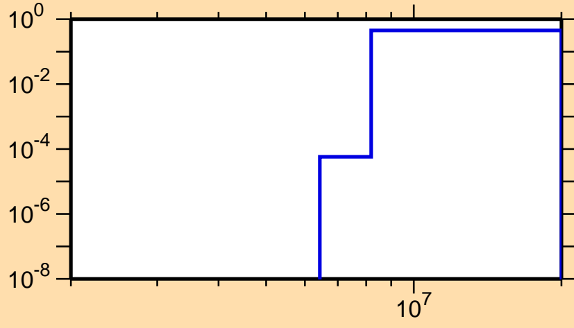
\sigma vs. E for ^{145}\text{Gd}(n,np)
