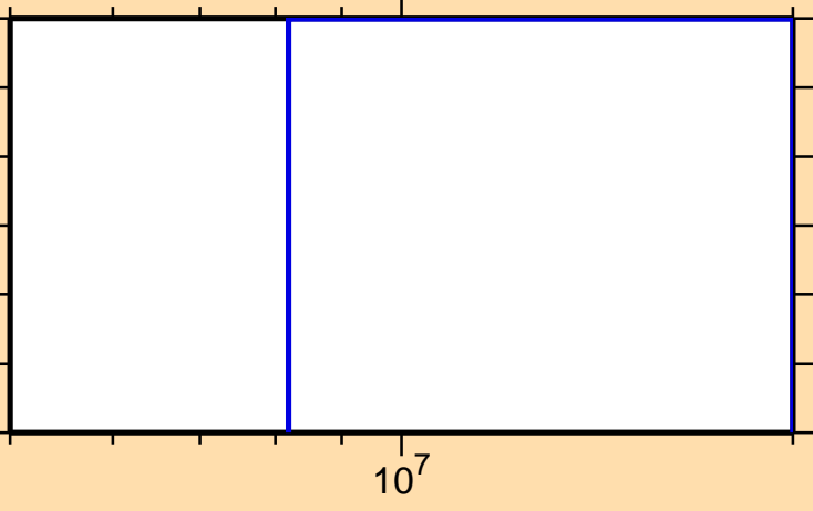
\sigma vs. E for ^{145}\text{Gd}(\text{mt117})
