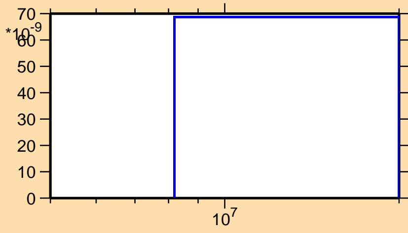
\sigma vs. E for ^{145}\text{Gd}(n,\text{pd})
