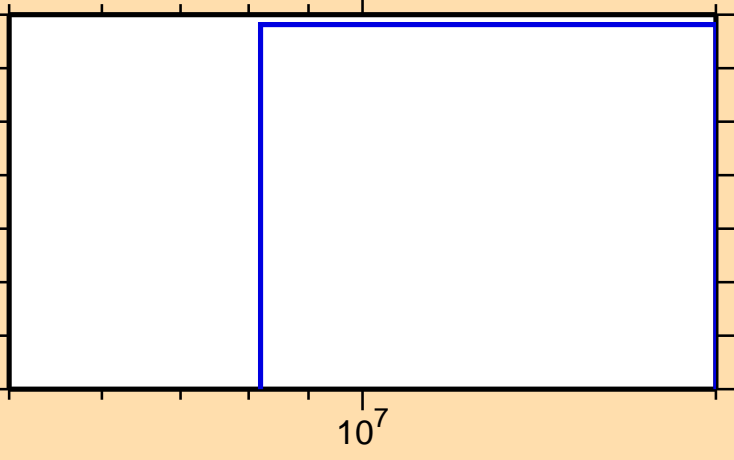
\sigma vs. E for ^{145}\text{Gd}(n,\text{nd})
