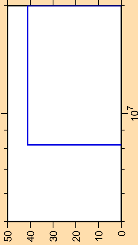
\Delta\sigma/\sigma vs. E for ^{145}\text{Gd}(n,\alpha)
