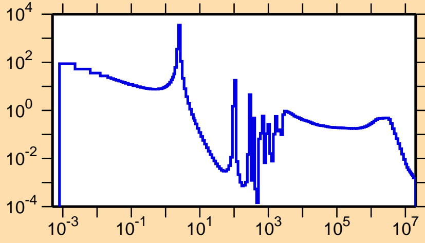
\sigma vs. E for ^{146}\text{Gd}(n,\gamma)
