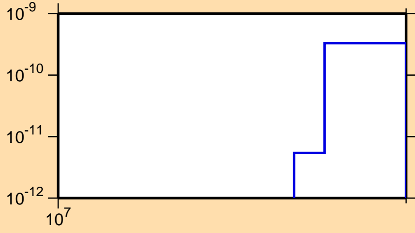
\sigma vs. E for ^{146}\text{Gd} (mt 45)
