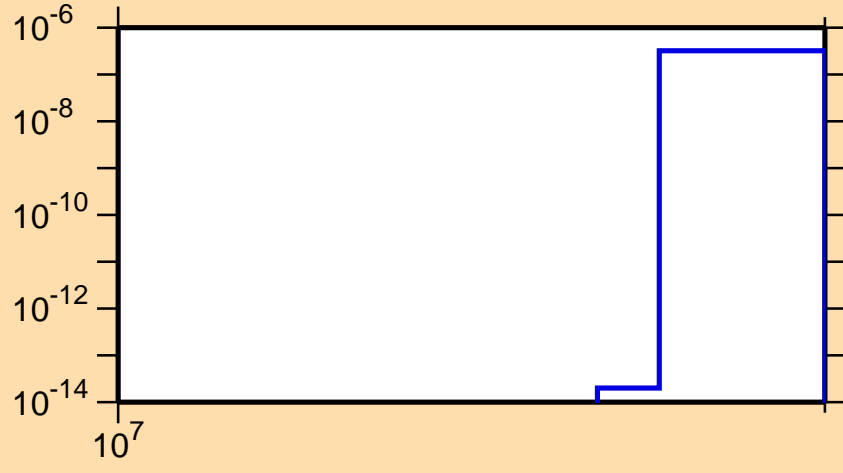
\sigma vs. E for ^{146}\text{Gd}(n,2np)
