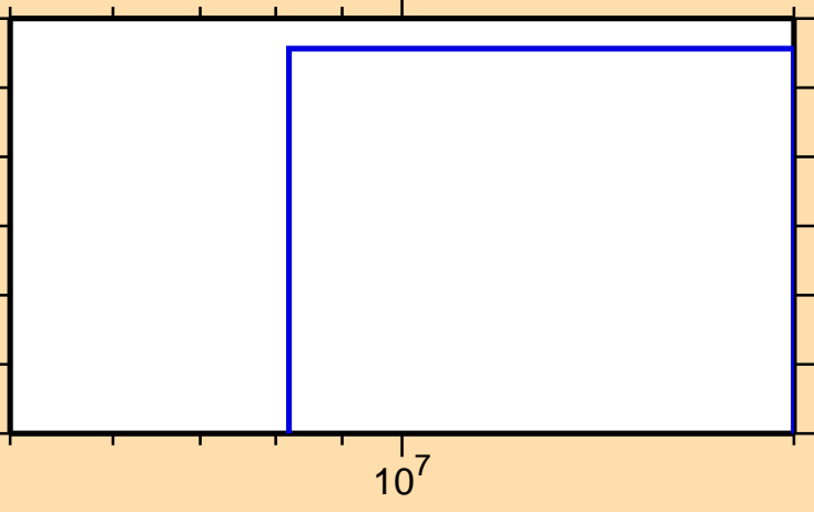
\sigma vs. E for ^{146}\text{Gd}(n,t)
