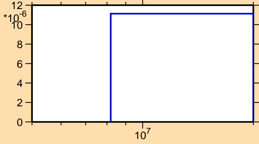
\sigma vs. E for ^{146}\text{Gd}(n,t)
