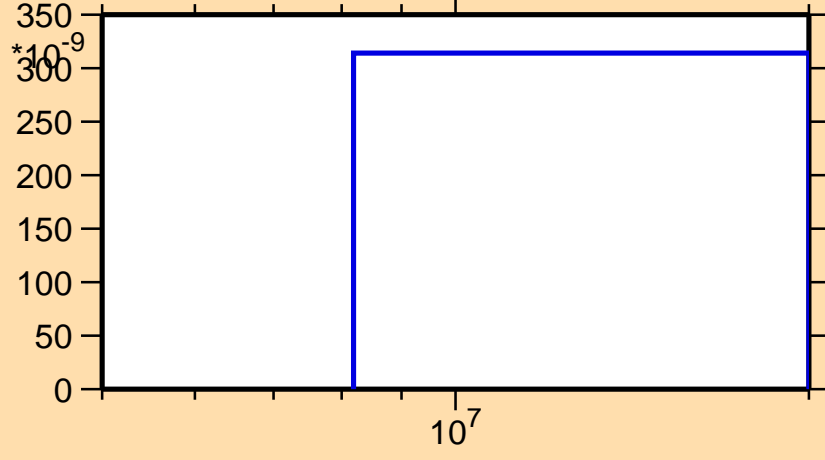
\sigma vs. E for ^{147}\text{Gd}(n,\text{nd})
