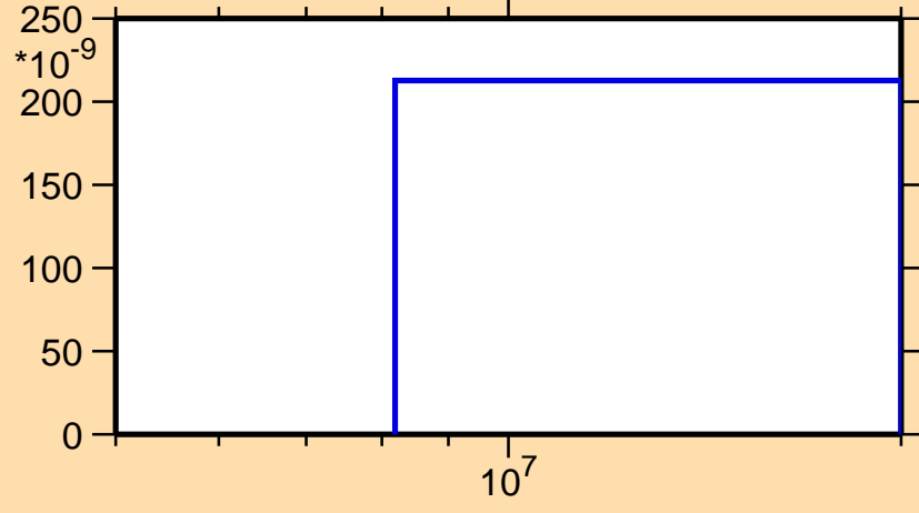
\sigma vs. E for ^{147}\text{Gd}(n,\text{He3})
