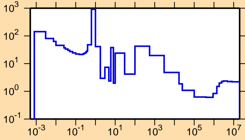
\sigma vs. E for ^{147}\text{Gd}(n,\text{nonel.})
