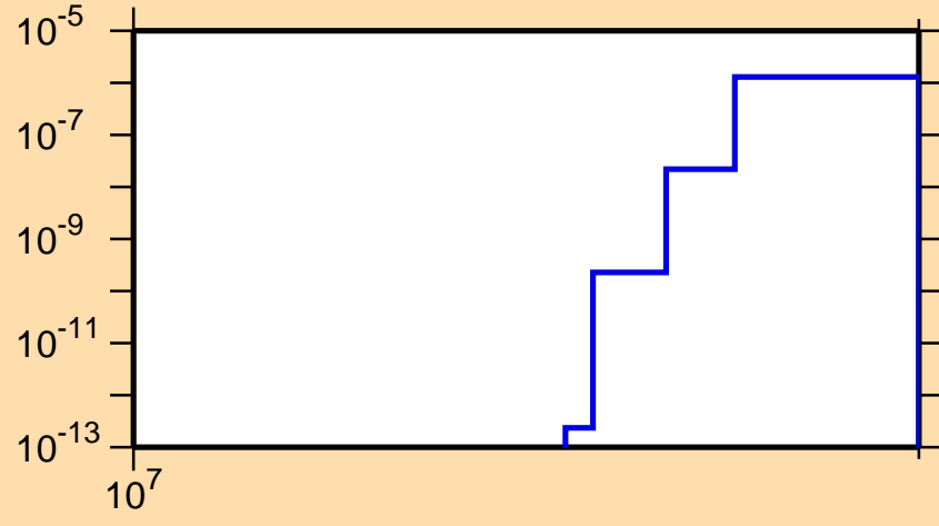
\sigma vs. E for ^{148}\text{Gd}(n,\text{nd})
