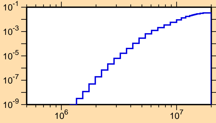
\sigma vs. E for ^{148}\text{Gd}(n,p)
