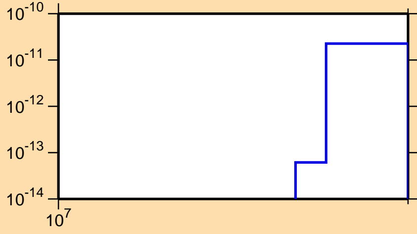
\sigma vs. E for ^{148}\text{Gd}(n,\text{pt})
