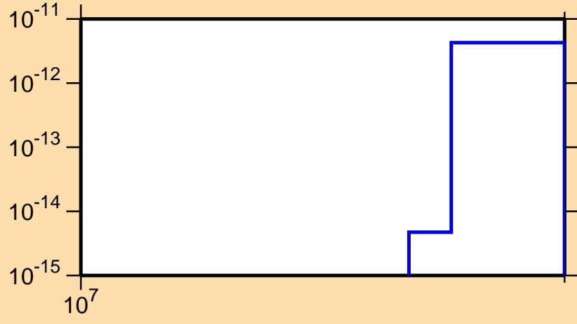
\sigma vs. E for ^{148}\text{Gd} (mt 34)
