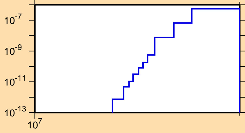
\sigma vs. E for ^{148}\text{Gd}(n,2n\alpha)
