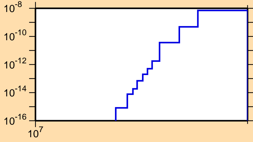
\sigma vs. E for ^{148}\text{Gd}(n,\text{pd})
