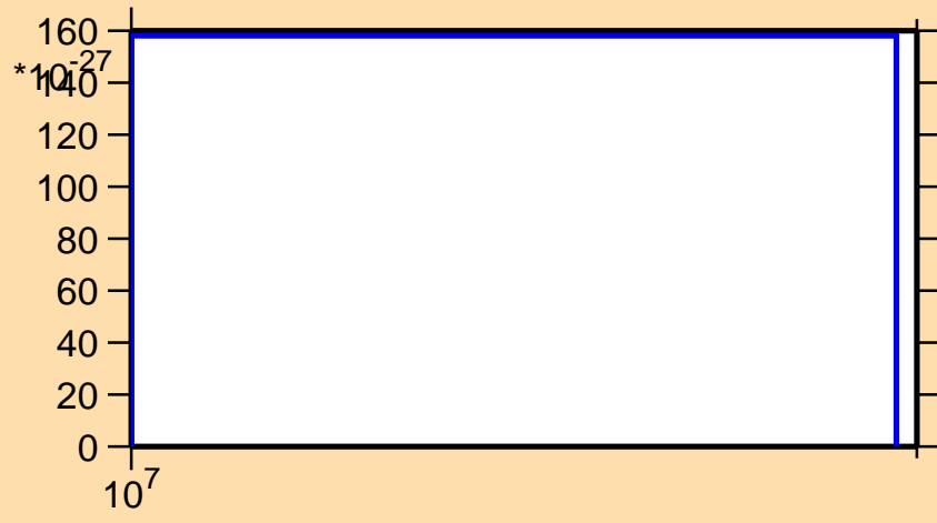
\sigma vs. E for ^{148}\text{Gd} (mt 11)
