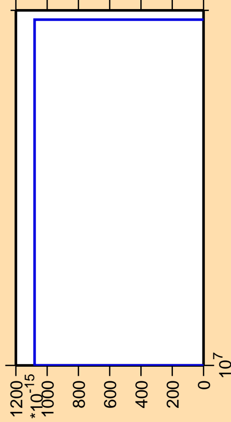
\Delta\sigma/\sigma vs. E for ^{148}\text{Gd} (mt 11)
