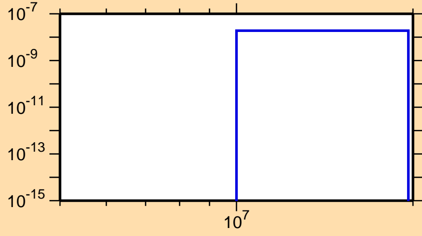
\sigma vs. E for ^{148}\text{Gd}(n,\text{He3})
