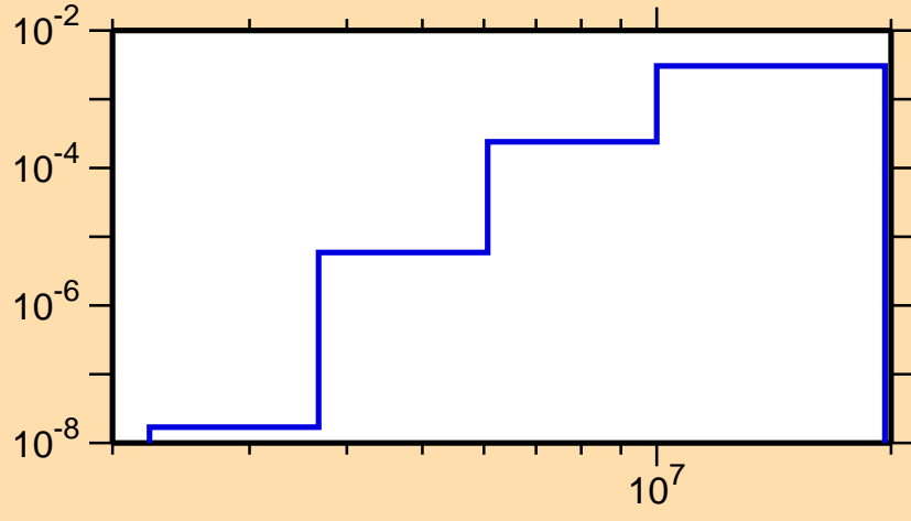
\sigma vs. E for ^{148}\text{Gd}(n,n\alpha)
