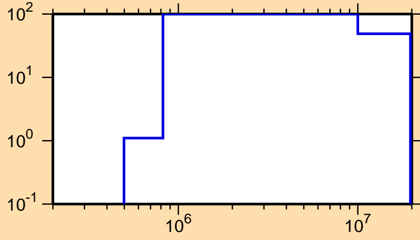
\Delta\sigma/\sigma vs. E for ^{148}\text{Gd}(n,p)
