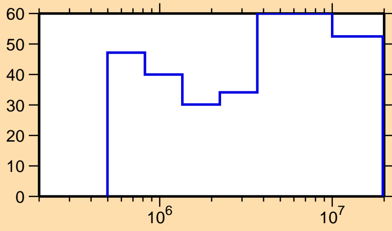
\Delta\sigma/\sigma vs. E for ^{148}\text{Gd}(n,n_1)
