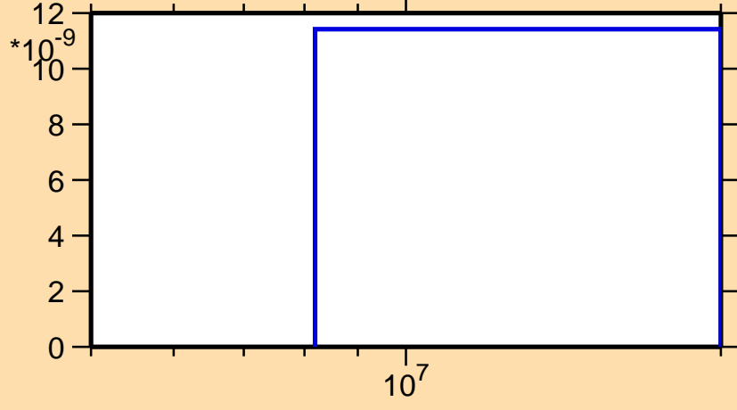
\sigma vs. E for ^{148}\text{Gd}(n,nd)
