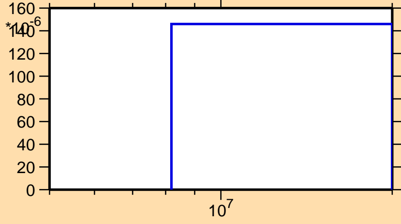
\sigma vs. E for ^{148}\text{Gd}(n,3n)
