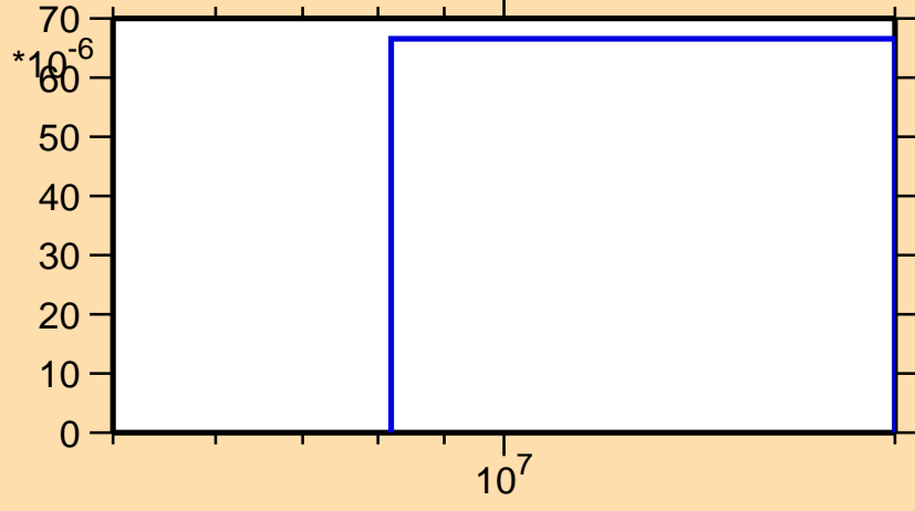
\sigma vs. E for ^{148}\text{Gd}(n,t)
