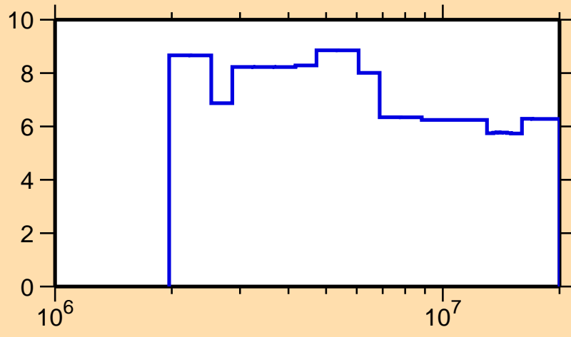
\Delta\sigma/\sigma vs. E for ^{149}\text{Gd}(n,n\text{onel.})
