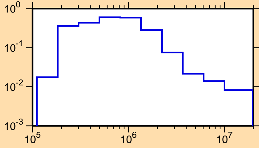
\sigma vs. E for ^{149}\text{Gd}(n,n_1)
