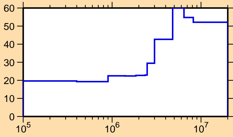
\Delta\sigma/\sigma vs. E for ^{149}\text{Gd}(n,n_1)
