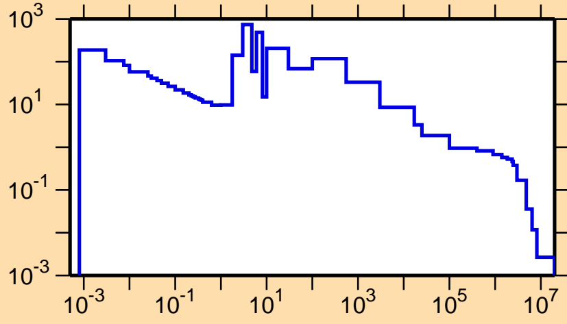
\sigma vs. E for ^{149}\text{Gd}(n,\gamma)
