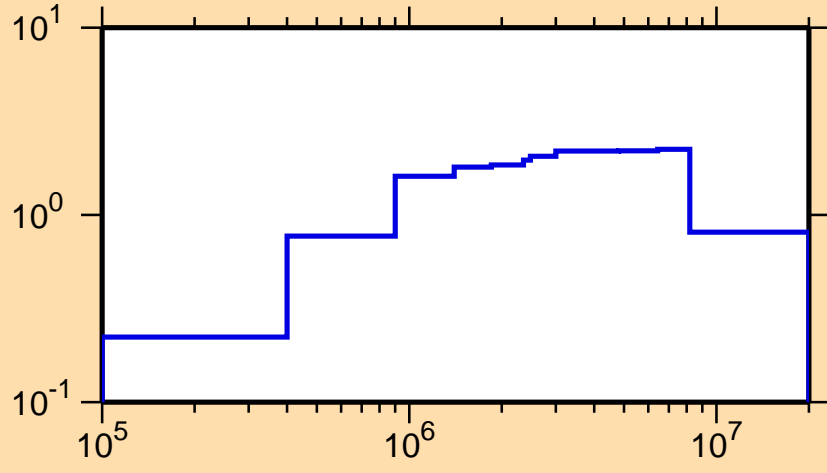
\sigma vs. E for ^{149}\text{Gd}(n,\text{inel.})
