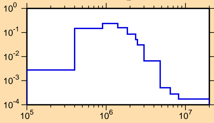
\sigma vs. E for ^{149}\text{Gd}(n,n_2)
