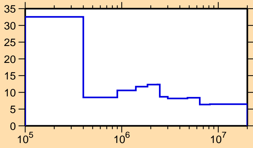
\Delta\sigma/\sigma vs. E for ^{149}\text{Gd}(n,\text{tot.})
