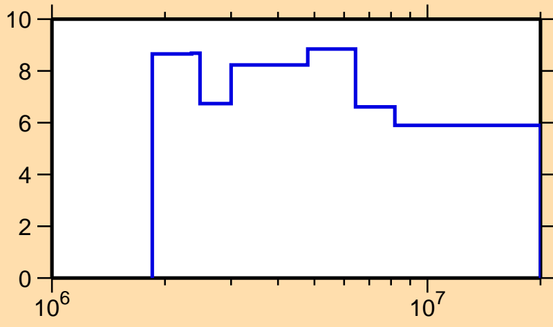
\Delta\sigma/\sigma vs. E for ^{149}\text{Gd}(n,\text{nonel.})
