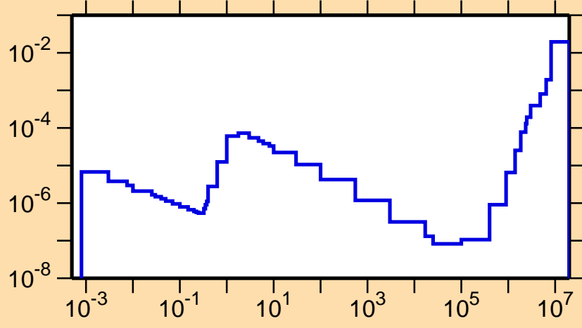
\sigma vs. E for ^{149}\text{Gd}(n,p)
