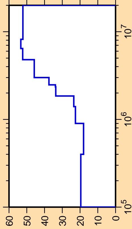
\Delta\sigma/\sigma vs. E for ^{149}\text{Gd}(n,n_2)
