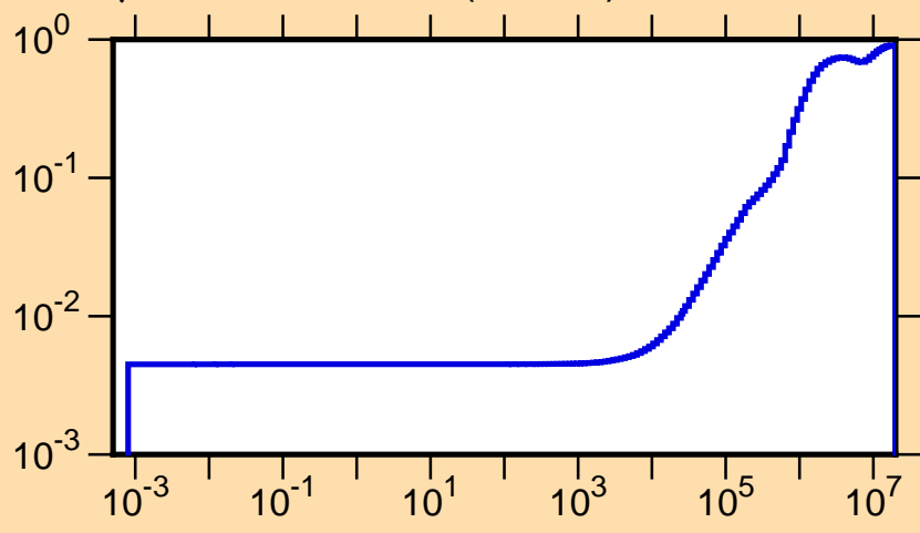
\mu vs. E for ^{150}\text{Gd}(\text{mt251})
