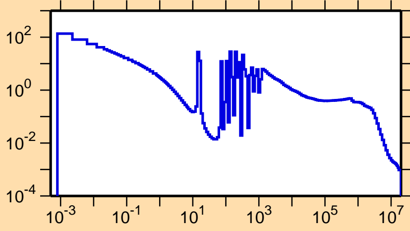
\sigma vs. E for ^{150}\text{Gd}(n,\gamma)
