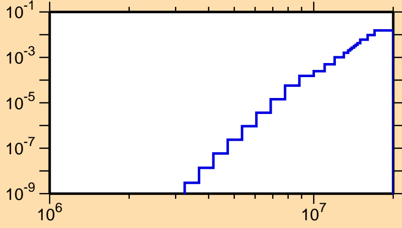
\sigma vs. E for ^{150}\text{Gd}(n,n\alpha)
