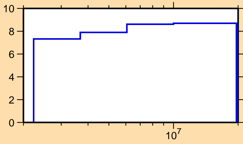
\Delta\sigma/\sigma vs. E for ^{150}\text{Gd}(n,n\text{nonel.})
