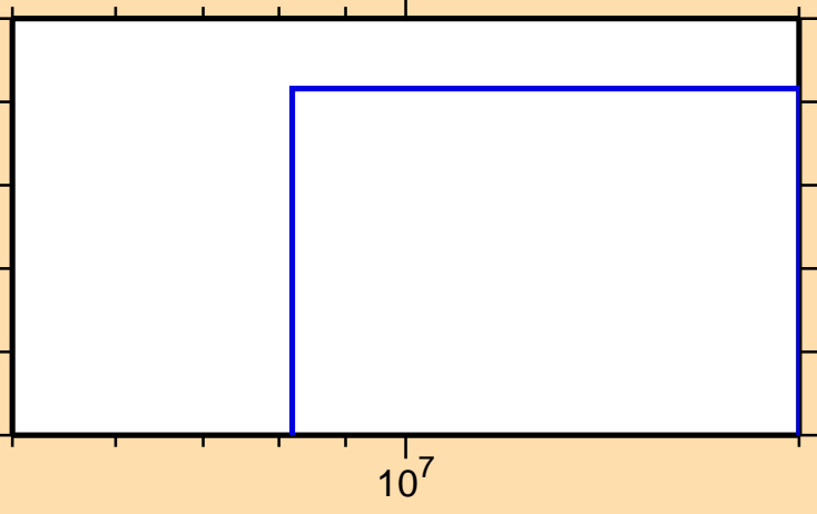
\sigma vs. E for ^{150}\text{Gd}(n,nd)
