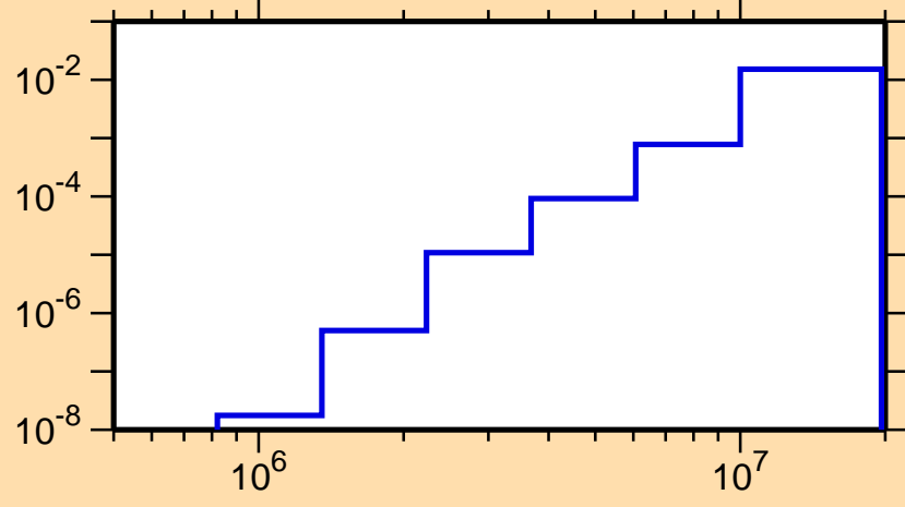
\sigma vs. E for ^{151}\text{Gd}(n,p)
