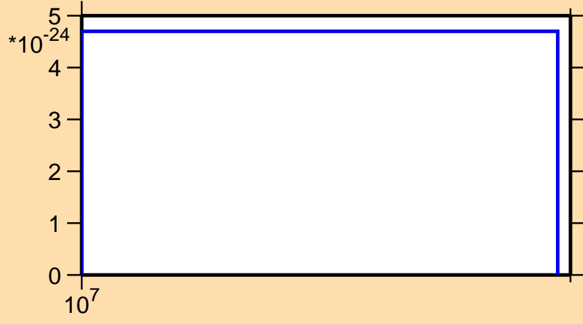
\sigma vs. E for ^{151}\text{Gd} (mt 11)
