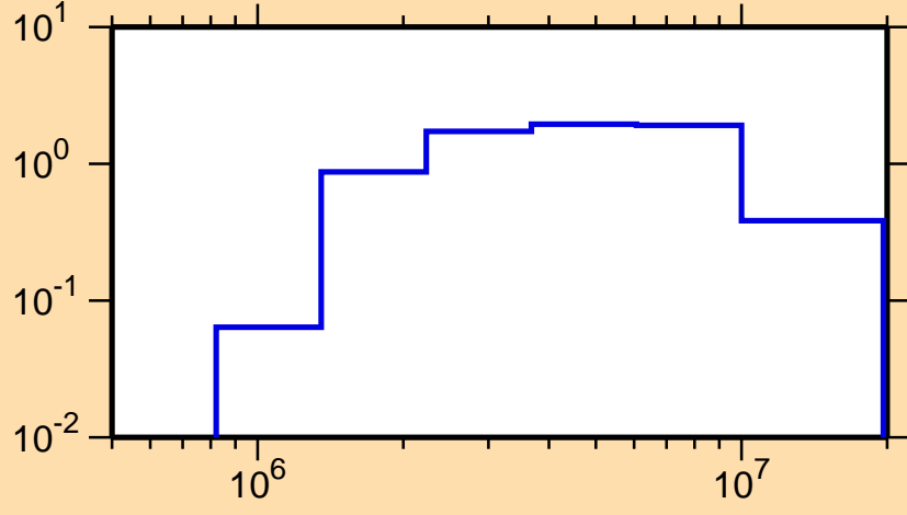
\sigma vs. E for ^{151}\text{Gd}(n,n\text{cont.})
