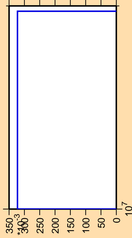
\Delta\sigma/\sigma vs. E for ^{151}\text{Gd} (mt 34)
