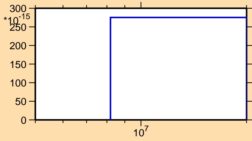
\sigma vs. E for ^{151}\text{Gd}(n,3n\alpha)
