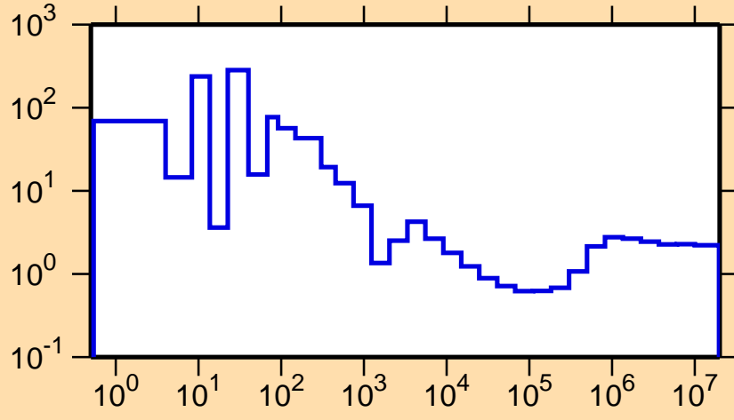
\sigma vs. E for ^{152}\text{Gd}(n,\text{nonel.})
