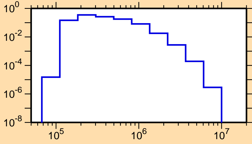
\sigma vs. E for ^{153}\text{Gd}(n,n_4)
