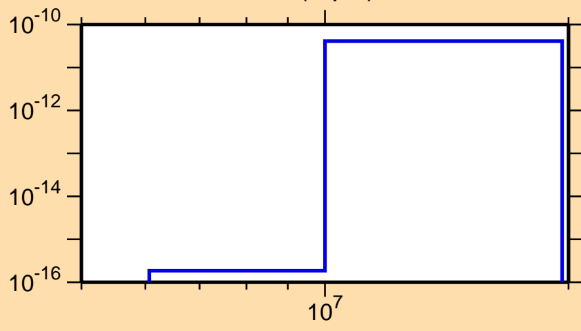
\sigma vs. E for ^{153}\text{Gd}(n,p\alpha)
