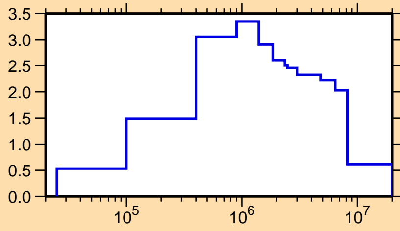
\sigma vs. E for ^{153}\text{Gd}(n,\text{inel.})
