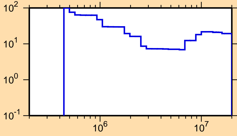
\Delta\sigma/\sigma vs. E for ^{155}\text{Gd}(n,n\text{cont.})
