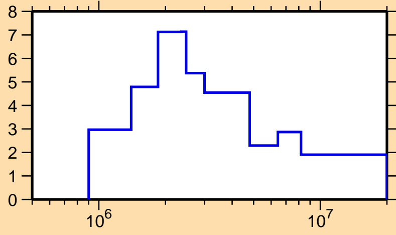
\Delta\sigma/\sigma vs. E for ^{155}\text{Gd}(n,\text{tot.})
