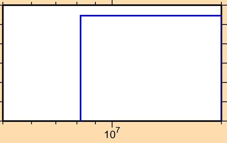
\sigma vs. E for ^{155}\text{Gd}(n,2n\alpha)
