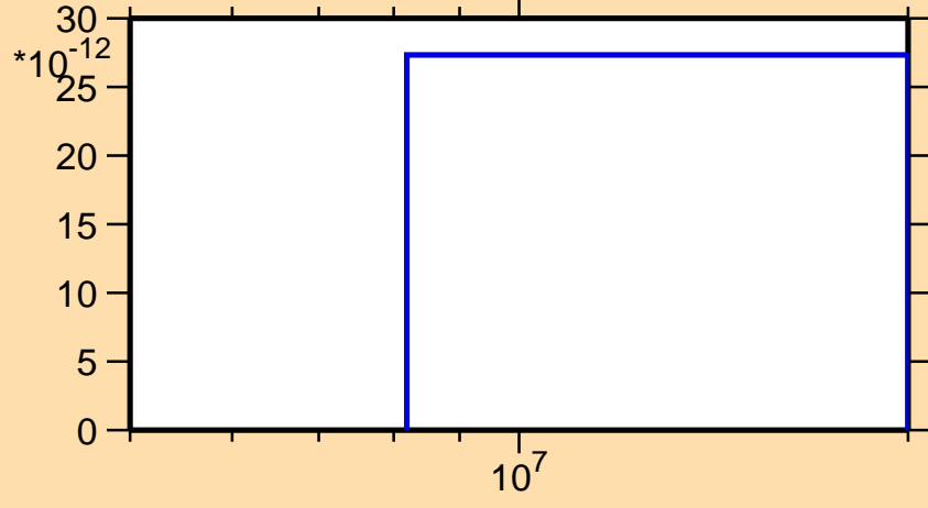
\sigma vs. E for ^{155}\text{Gd}(n,nt)
