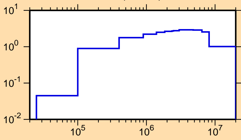
\sigma vs. E for ^{155}\text{Gd}(n,\text{inel.})
