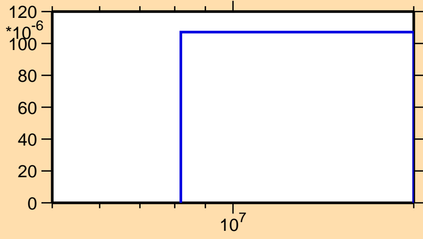
\sigma vs. E for ^{155}\text{Gd}(n,t)
