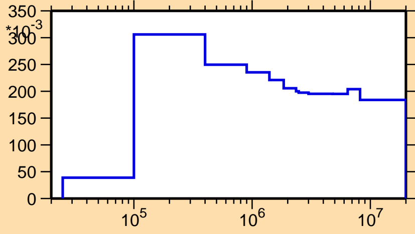
\sigma vs. E for ^{155}\text{Gd}(n,n_1)
