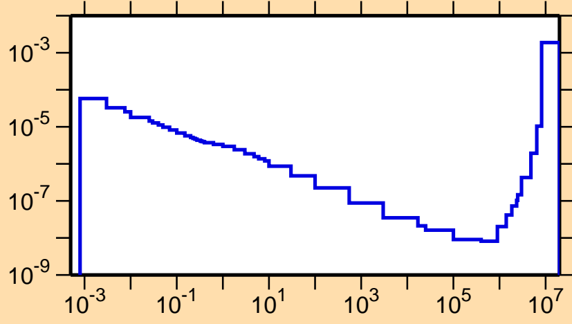
\sigma vs. E for ^{155}\text{Gd}(n,\alpha)
