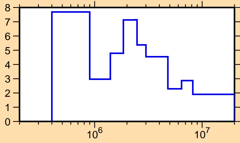
\Delta\sigma/\sigma vs. E for ^{155}\text{Gd}(n,tot.)
