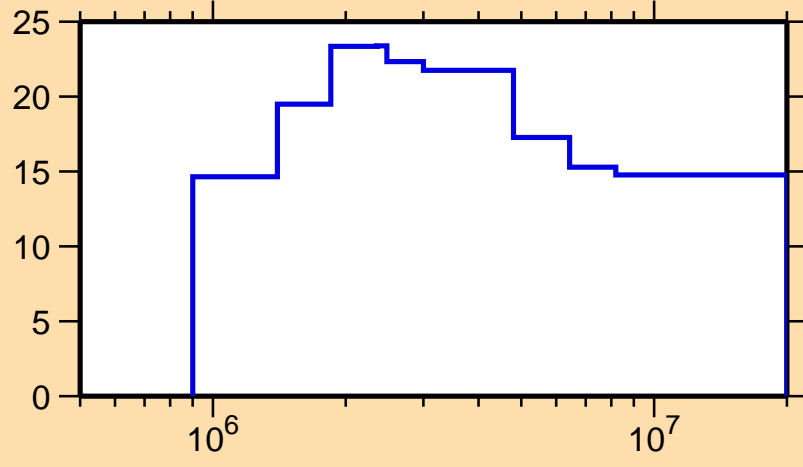
\Delta\sigma/\sigma vs. E for ^{155}\text{Gd}(n,n_1)
