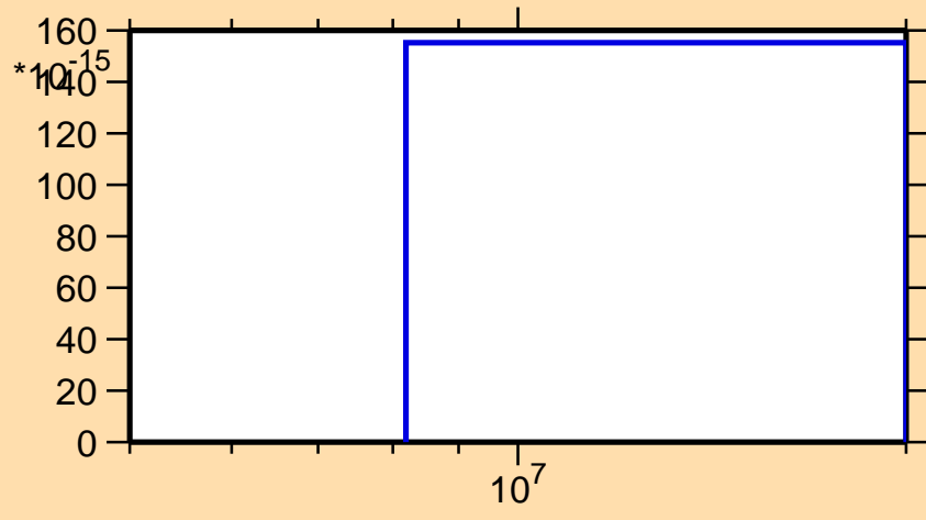
\sigma vs. E for ^{155}\text{Gd}(n,p\alpha)
