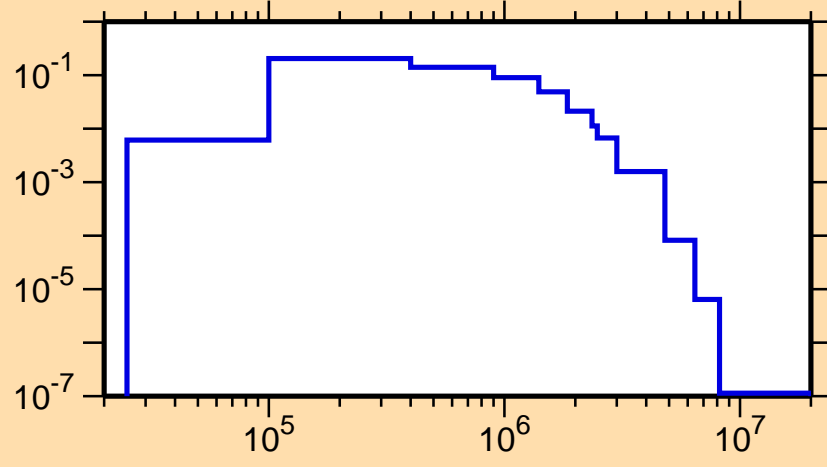
\sigma vs. E for ^{155}\text{Gd}(n,n_2)
