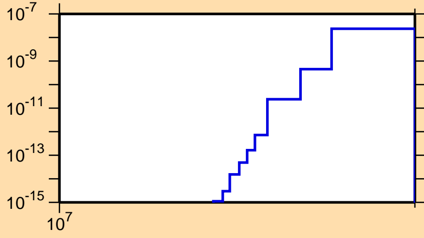
\sigma vs. E for ^{156}\text{Gd}(n,2n\alpha)
