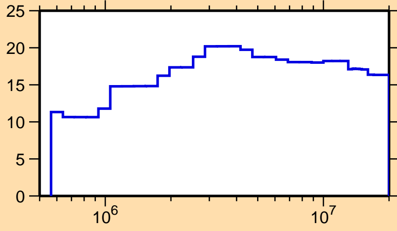
\Delta\sigma/\sigma vs. E for ^{156}\text{Gd}(n,n_1)
