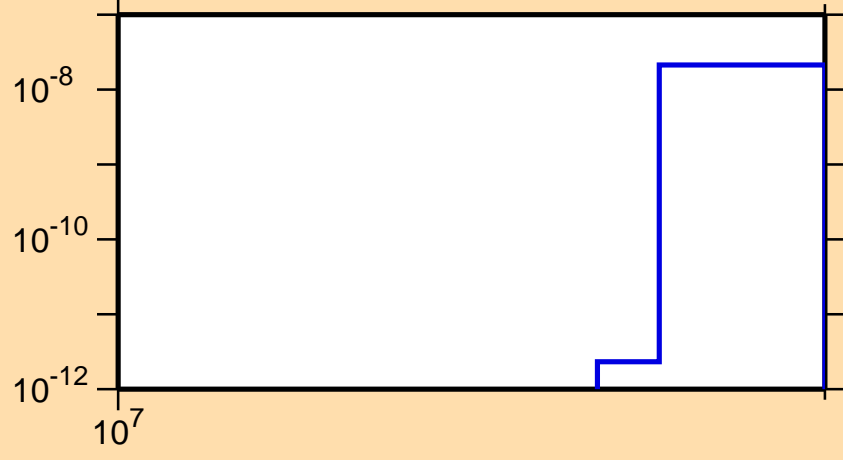
\sigma vs. E for ^{156}\text{Gd}(n,\text{nd})
