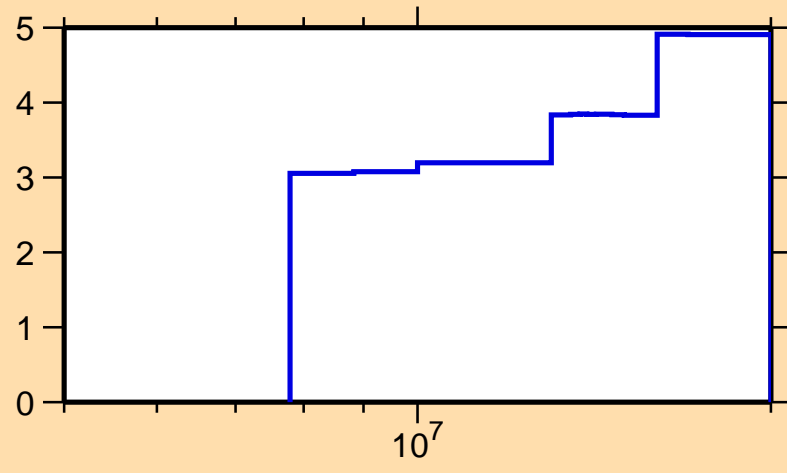
\Delta\sigma/\sigma vs. E for ^{156}\text{Gd}(n,\text{tot.})
