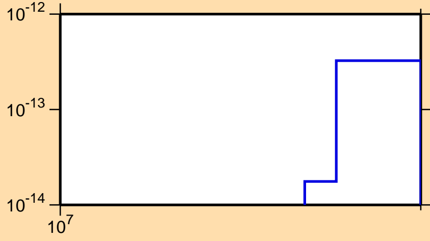
\sigma vs. E for ^{156}\text{Gd}(n,p\alpha)
