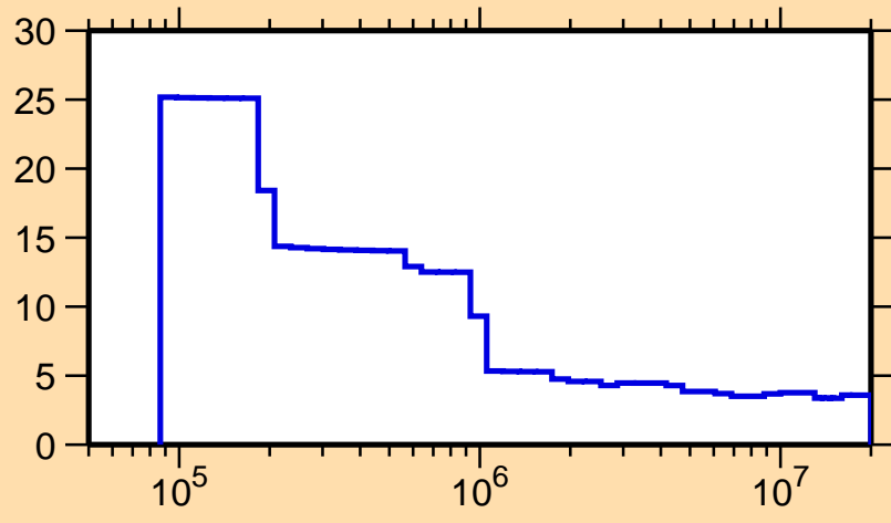
\Delta\sigma/\sigma vs. E for ^{156}\text{Gd}(n,\text{nonel.})
