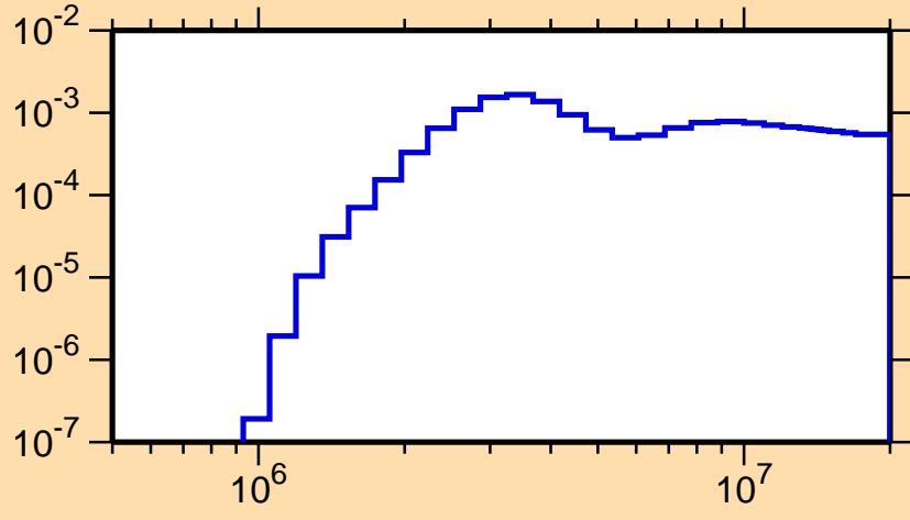
\sigma vs. E for ^{156}\text{Gd}(n,n_4)
