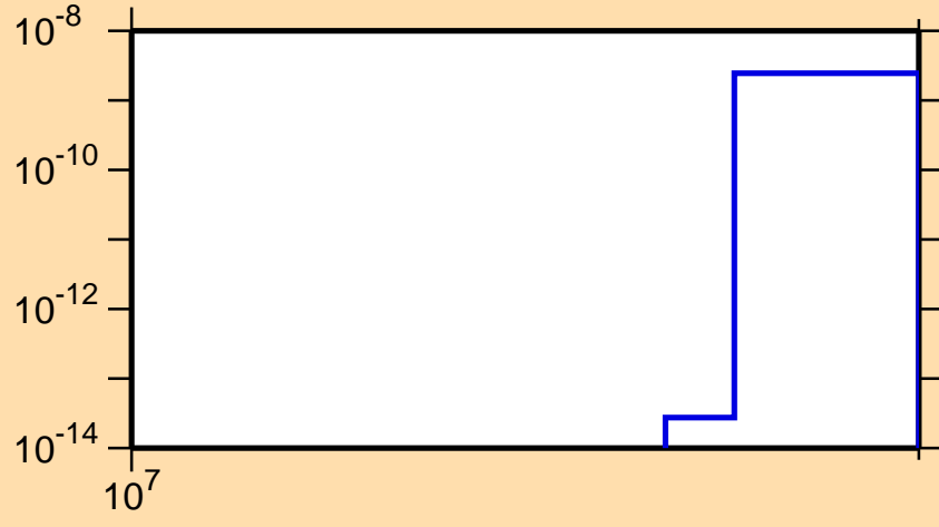
\sigma vs. E for ^{156}\text{Gd}(n,nt)
