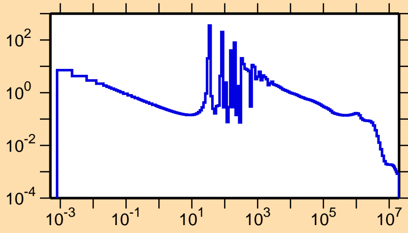
\sigma vs. E for ^{156}\text{Gd}(n,\gamma)
