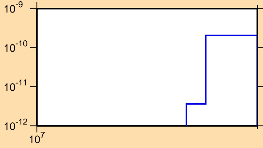
\sigma vs. E for ^{156}\text{Gd}(n,\text{He3})
