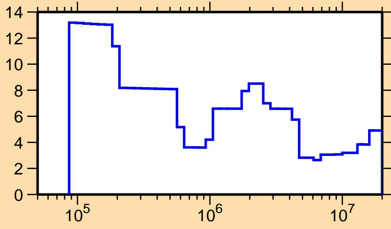
\Delta\sigma/\sigma vs. E for ^{156}\text{Gd}(n,\text{tot.})
