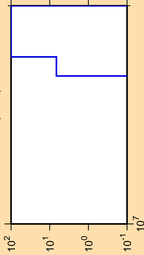
\Delta\sigma/\sigma vs. E for ^{156}\text{Gd}(n,\text{nd})
