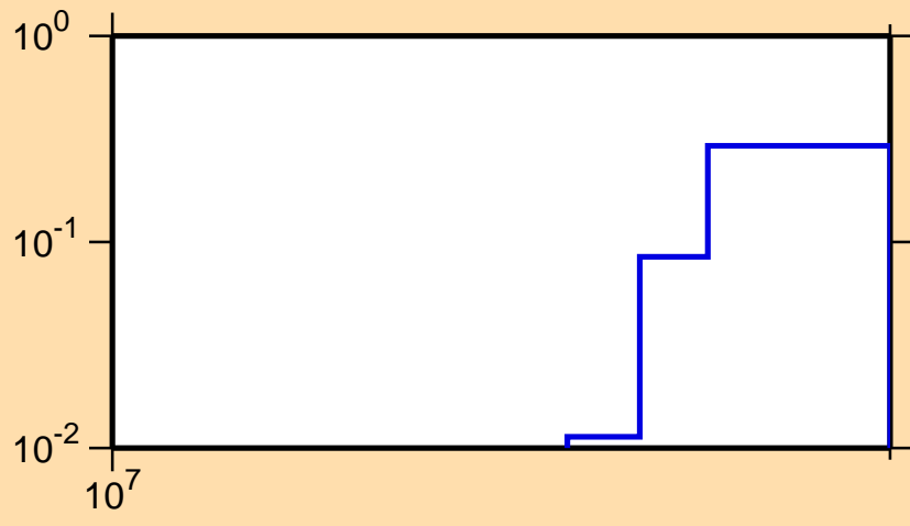
\sigma vs. E for ^{156}\text{Gd}(n,3n)
