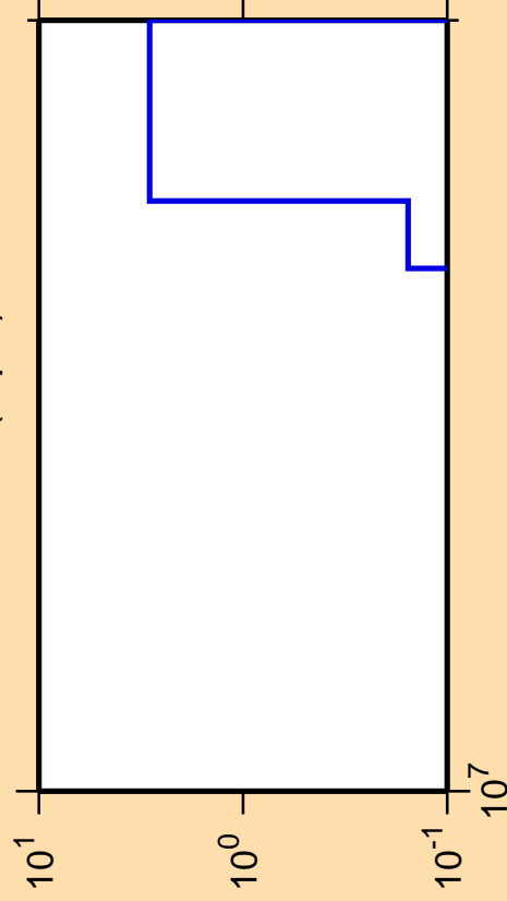
\Delta\sigma/\sigma vs. E for ^{156}\text{Gd}(n,p\alpha)
