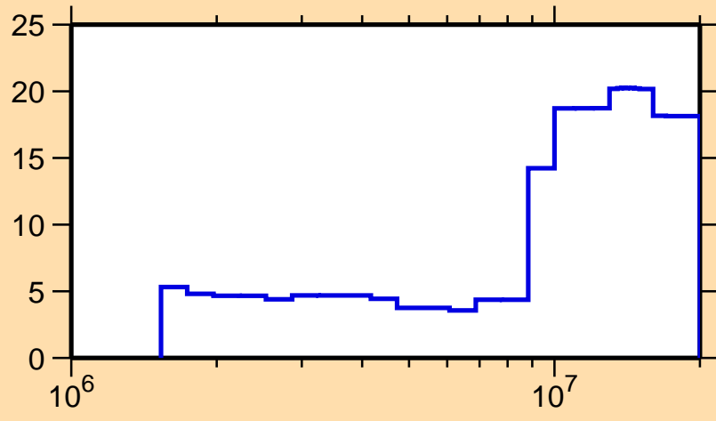
\Delta\sigma/\sigma vs. E for ^{156}\text{Gd}(n,\text{inel.})
