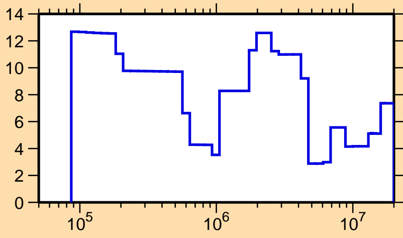
\Delta\sigma/\sigma vs. E for ^{156}\text{Gd}(n,\text{el.})
