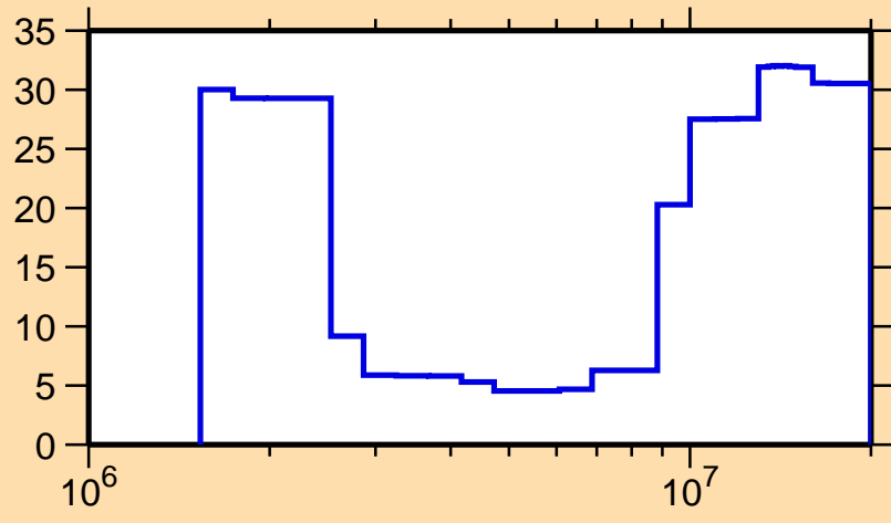
\Delta\sigma/\sigma vs. E for ^{156}\text{Gd}(n,n\text{cont.})
