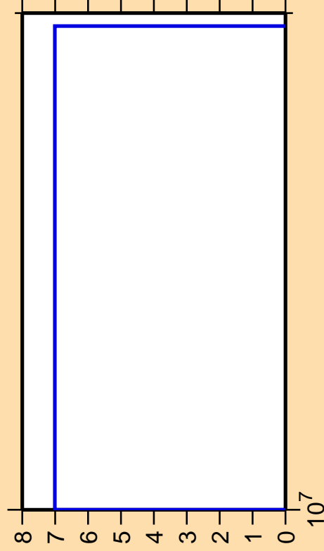
\Delta\sigma/\sigma vs. E for ^{156}\text{Gd}(n,\text{He3})
