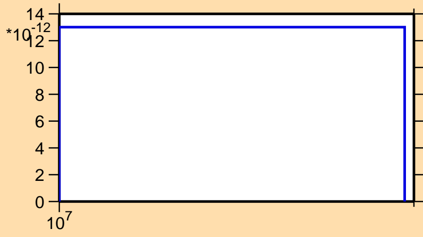
\sigma vs. E for ^{156}\text{Gd}(n,2np)
