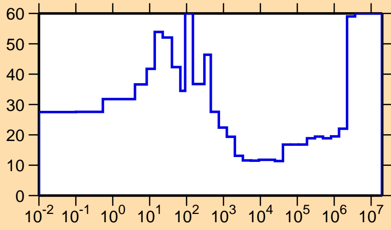
\Delta\sigma/\sigma vs. E for ^{156}\text{Gd}(n,\gamma)
