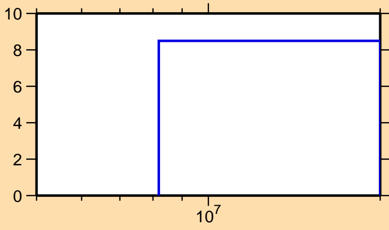
\Delta\sigma/\sigma vs. E for ^{156}\text{Gd}(n,2n)
