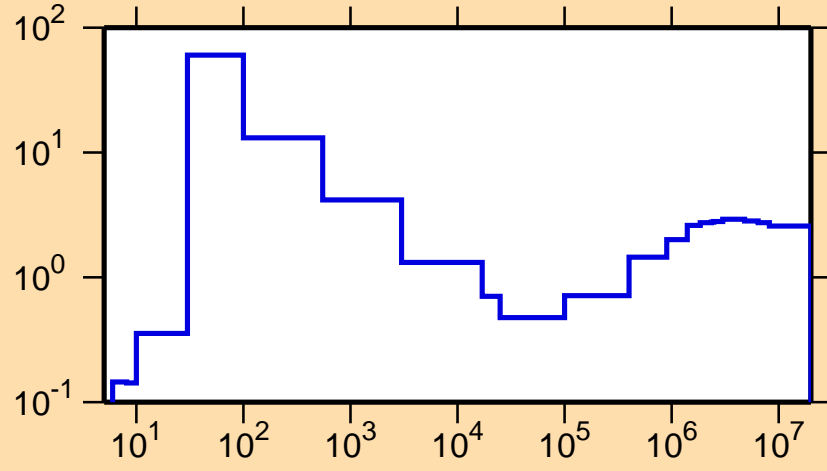
\sigma vs. E for ^{156}\text{Gd}(n,\text{nonel.})
