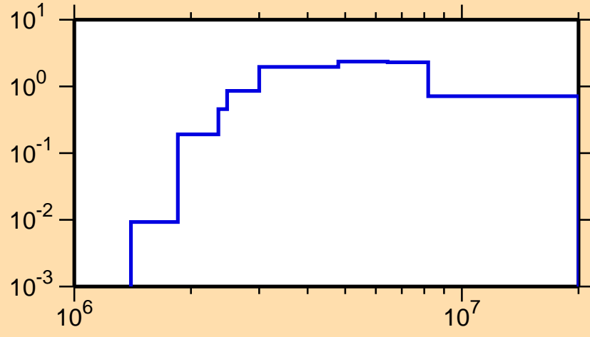
\sigma vs. E for ^{156}\text{Gd}(n,n\text{cont.})
