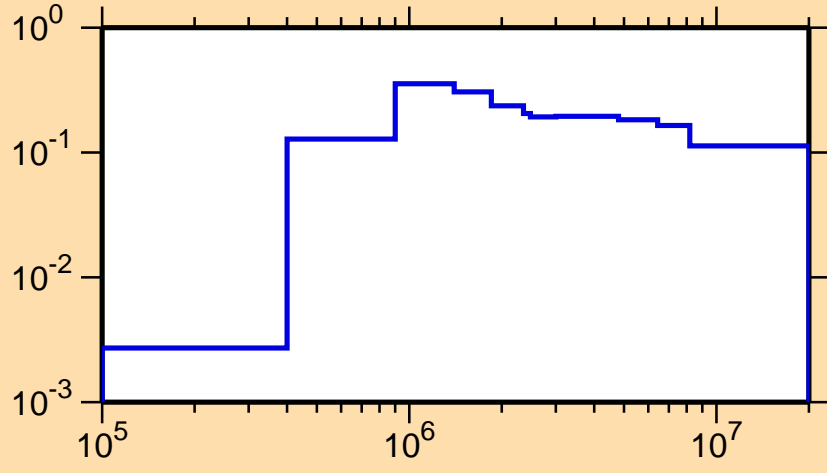
\sigma vs. E for ^{158}\text{Gd}(n,n_2)
