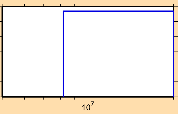
\sigma vs. E for ^{158}\text{Gd}(n,t)
