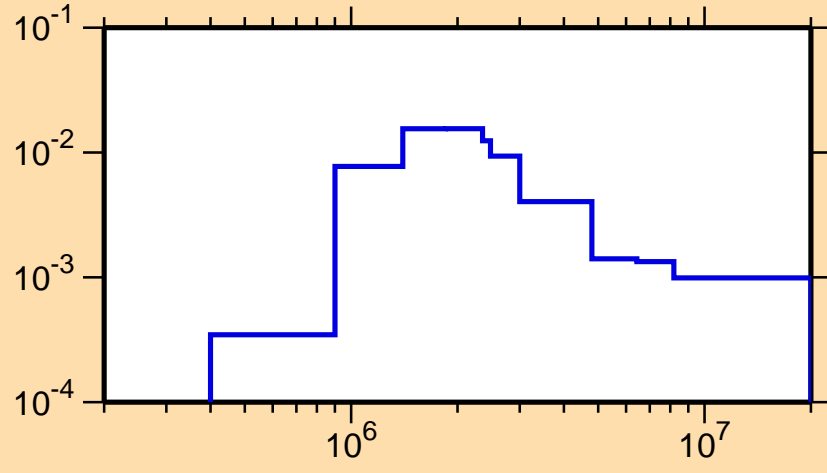
\sigma vs. E for ^{158}\text{Gd}(n,n_3)
