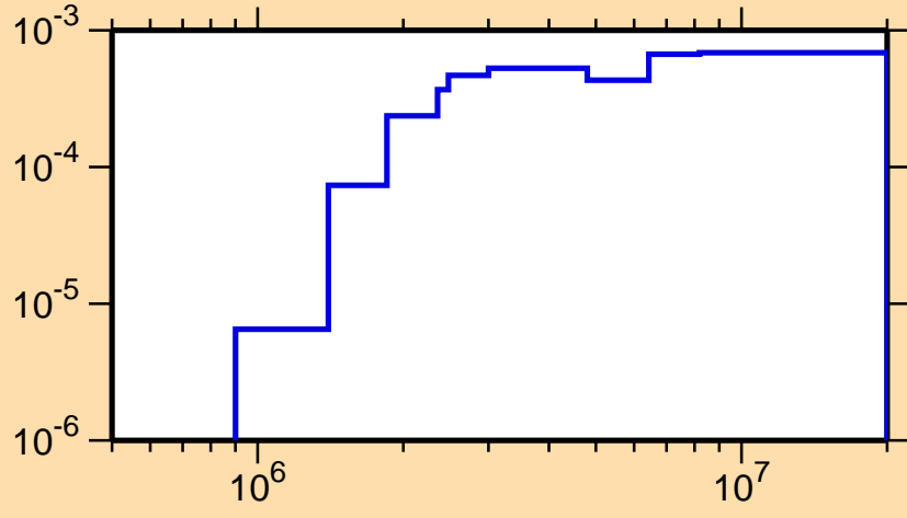
\sigma vs. E for ^{158}\text{Gd}(n,n_4)
