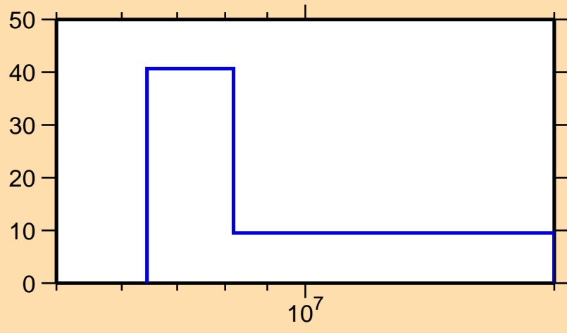
\Delta\sigma/\sigma vs. E for ^{158}\text{Gd}(n,2n)
