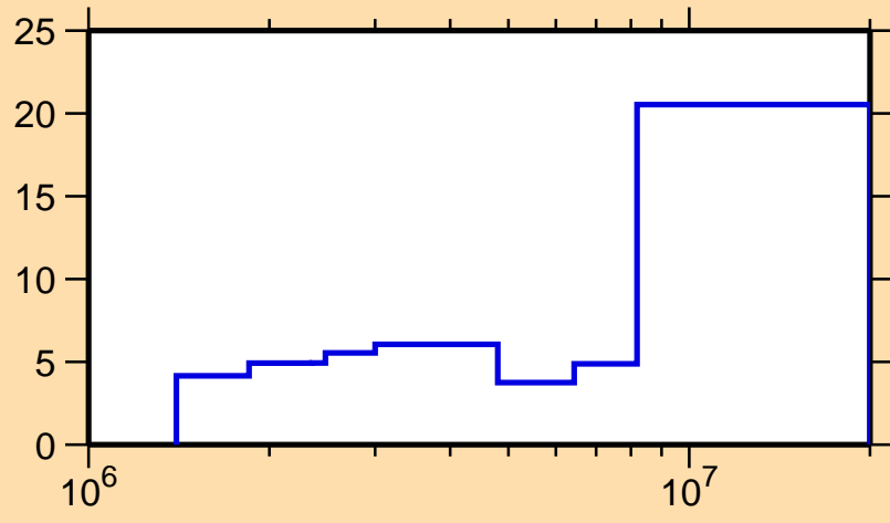
\Delta\sigma/\sigma vs. E for ^{158}\text{Gd}(n,\text{inel.})
