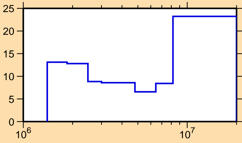
\Delta\sigma/\sigma vs. E for ^{158}\text{Gd}(n,n\text{cont.})
