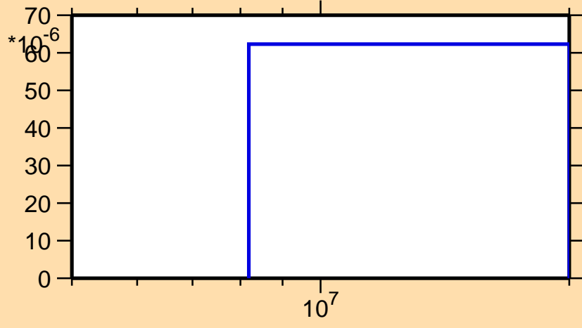
\sigma vs. E for ^{158}\text{Gd}(n,np)
