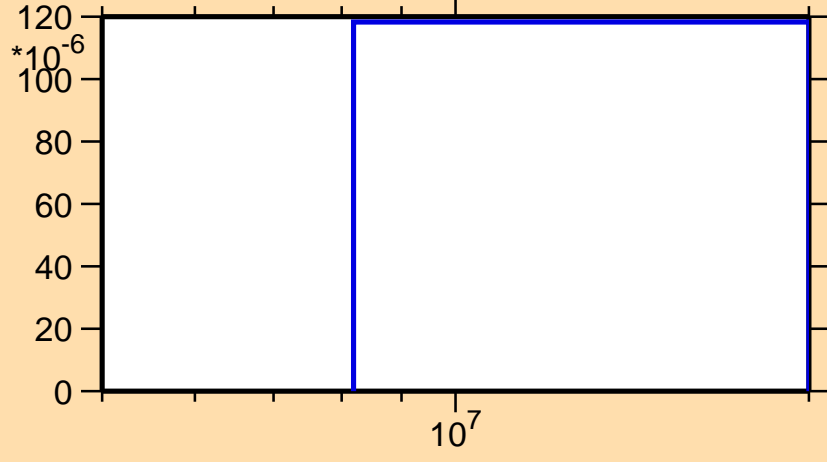
\sigma vs. E for ^{158}\text{Gd}(n,d)
