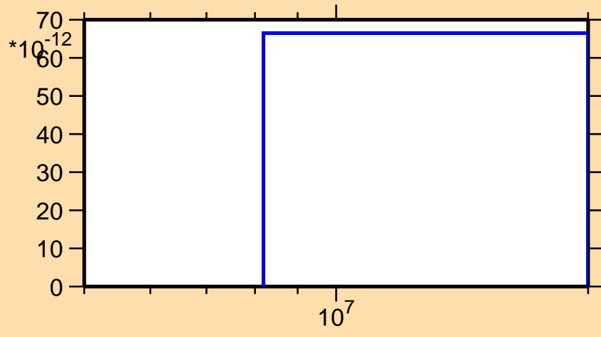
\sigma vs. E for ^{158}\text{Gd}(n,2n\alpha)
