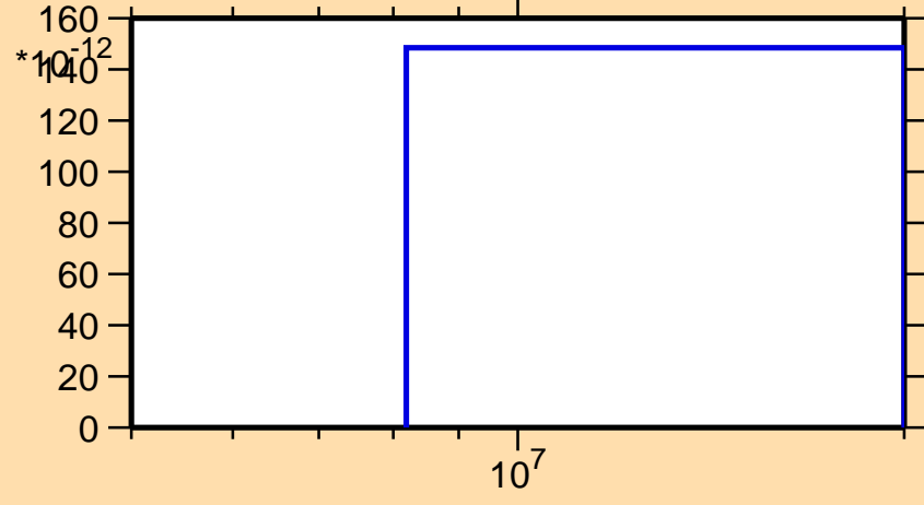
\sigma vs. E for ^{158}\text{Gd}(n,nd)
