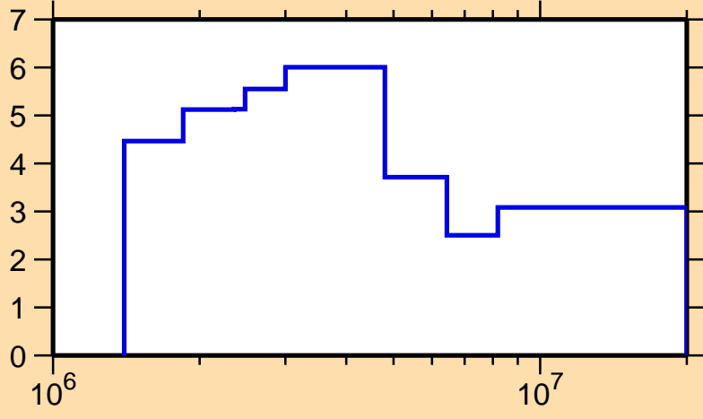
\Delta\sigma/\sigma vs. E for ^{158}\text{Gd}(n,n\text{onel.})
