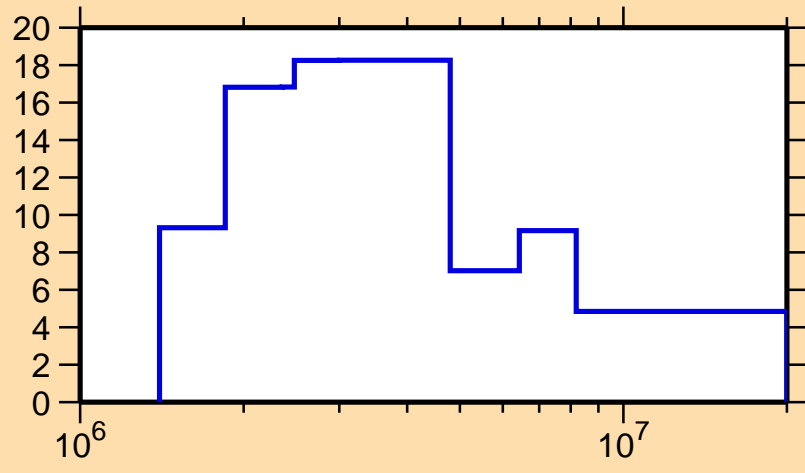
\Delta\sigma/\sigma vs. E for ^{158}\text{Gd}(n,\text{el.})
