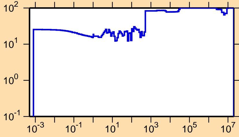
\Delta\sigma/\sigma vs. E for ^{159}\text{Gd}(n,\gamma)
