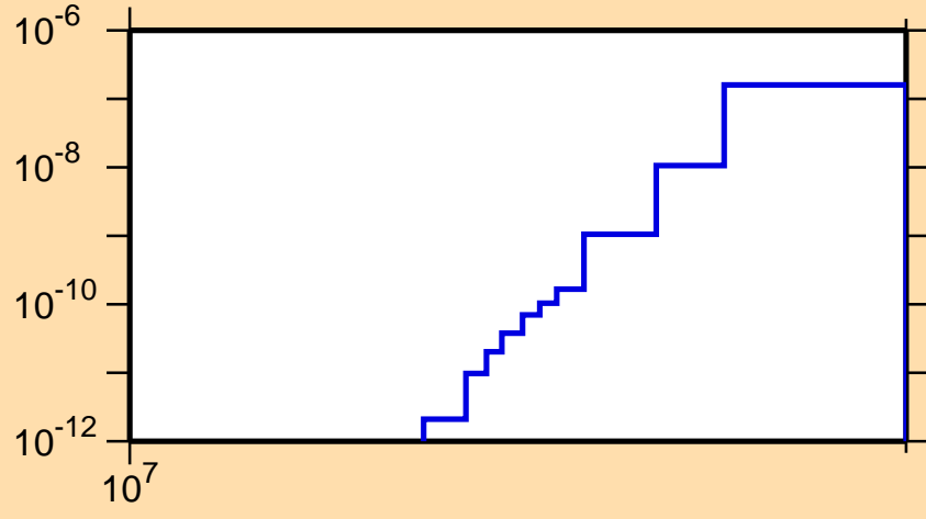
\sigma vs. E for ^{159}\text{Gd}(n,2n\alpha)
