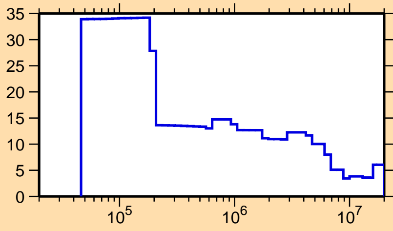
\Delta\sigma/\sigma vs. E for ^{159}\text{Gd}(n,\text{tot.})
