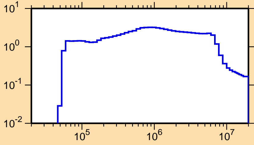
\sigma vs. E for ^{159}\text{Gd}(n,\text{inel.})
