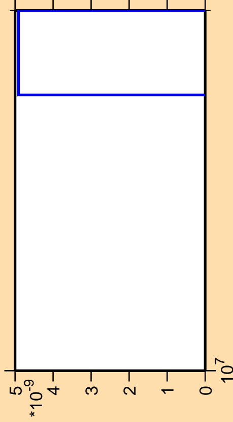
\Delta\sigma/\sigma vs. E for ^{159}\text{Gd} (mt 11)
