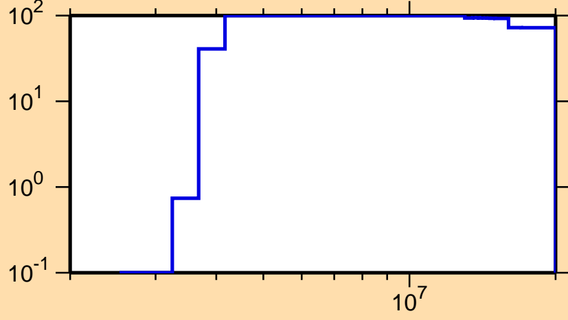
\Delta\sigma/\sigma vs. E for ^{159}\text{Gd}(n,p)
