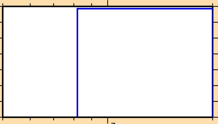
\sigma vs. E for ^{159}\text{Gd}(n,2np)
