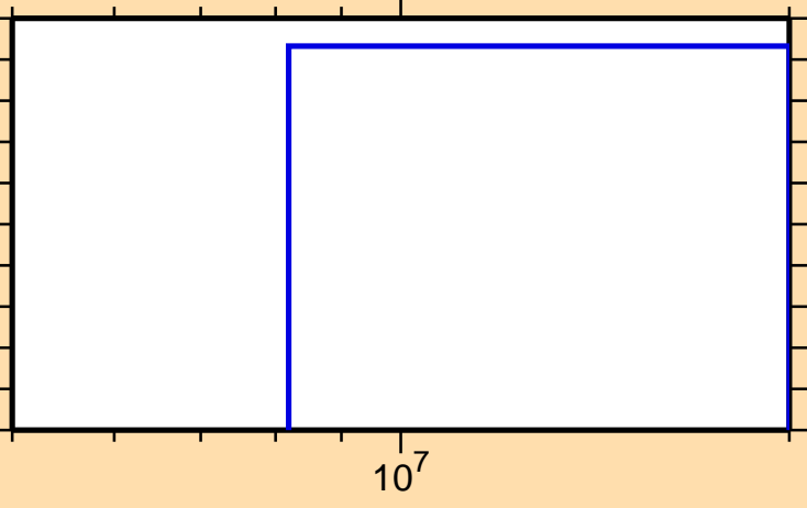
\sigma vs. E for ^{159}\text{Gd}(n,2n\alpha)
