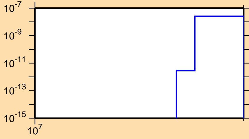
\sigma vs. E for ^{160}\text{Gd}(n,\text{nd})
