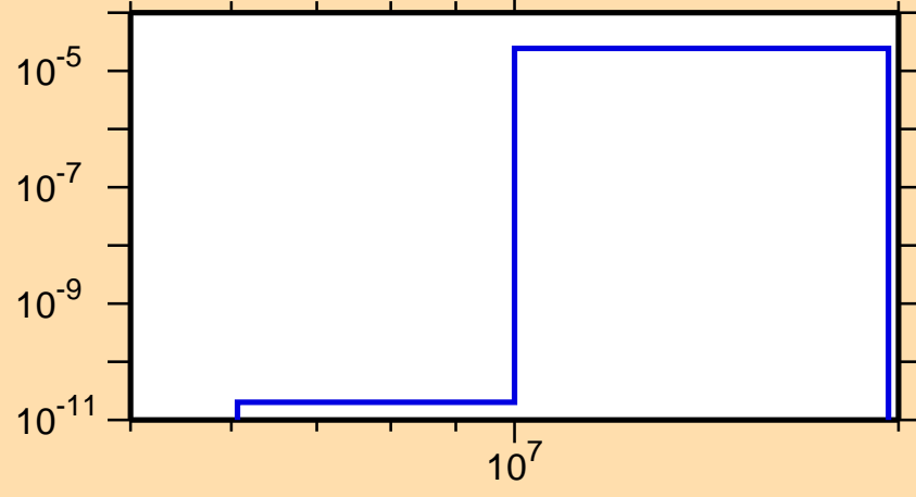
\sigma vs. E for ^{160}\text{Gd}(n,n\alpha)
