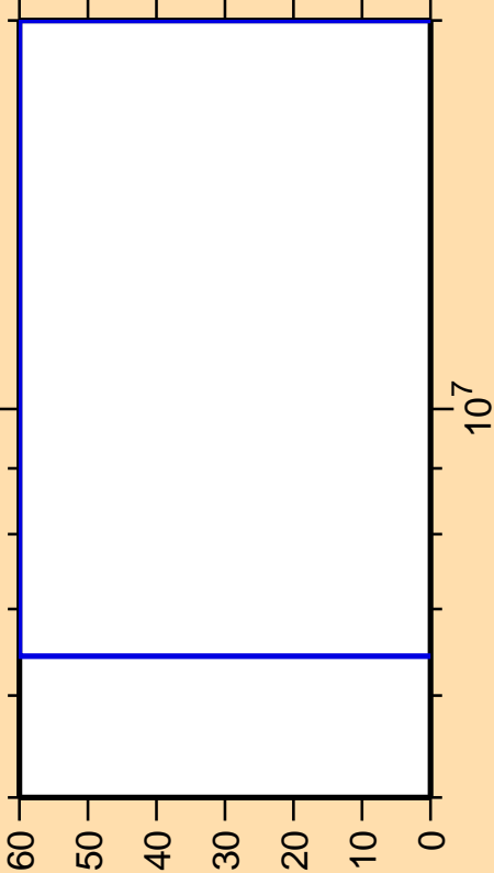
\Delta\sigma/\sigma vs. E for ^{160}\text{Gd}(n,\gamma)
