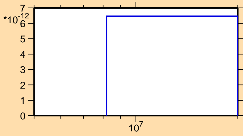
\sigma vs. E for ^{160}\text{Gd}(n,2np)
