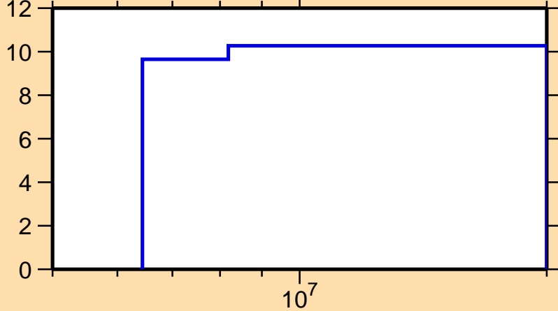
\Delta\sigma/\sigma vs. E for ^{160}\text{Gd}(n,2n)
