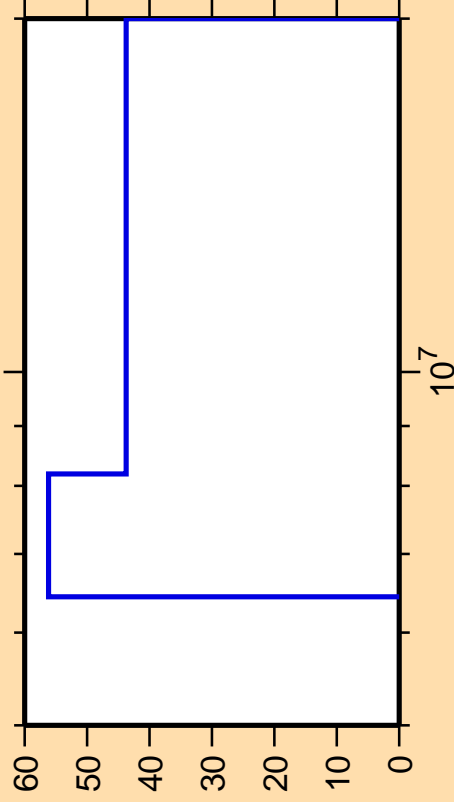
\Delta\sigma/\sigma vs. E for ^{160}\text{Gd}(n,\alpha)
