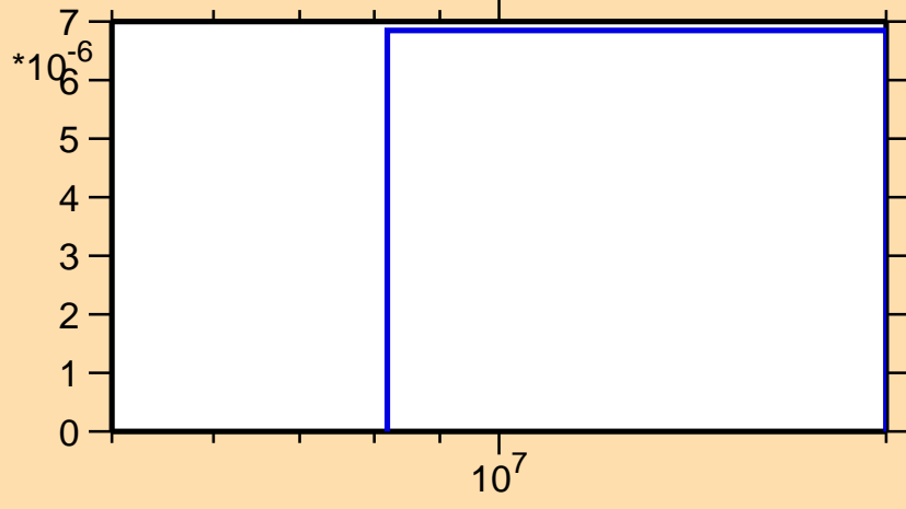
\sigma vs. E for ^{160}\text{Gd}(n,t)
