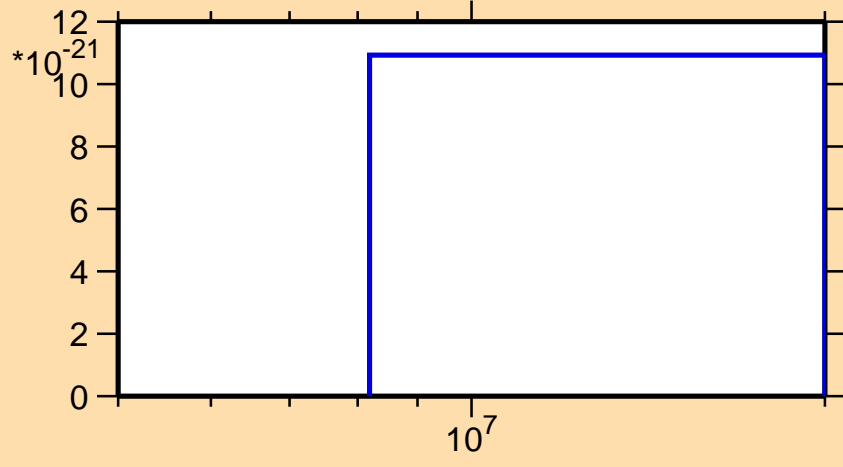
\sigma vs. E for ^{160}\text{Gd} (mt 11)
