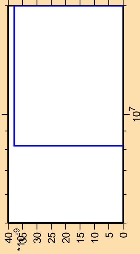
\Delta\sigma/\sigma vs. E for ^{160}\text{Gd} (mt 11)
