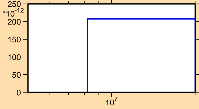
\sigma vs. E for ^{160}\text{Gd}(n,nd)
