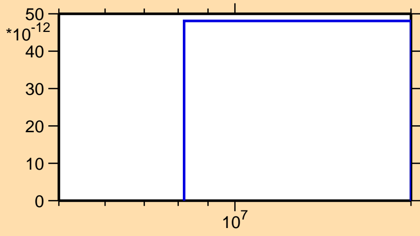
\sigma vs. E for ^{160}\text{Gd}(n,2n\alpha)
