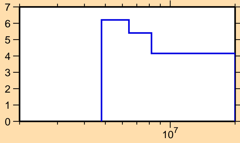
\Delta\sigma/\sigma vs. E for ^{161}\text{Gd}(n,2n)
