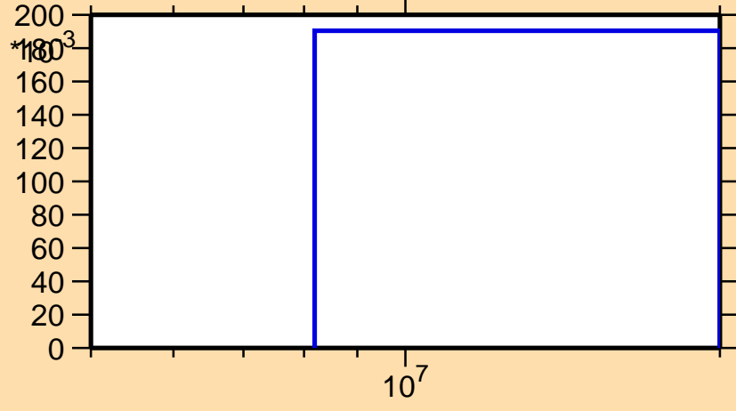
\sigma vs. E for ^{161}\text{Gd}(n,3n)
