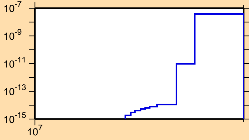
\sigma vs. E for ^{162}\text{Gd}(n,nt)
