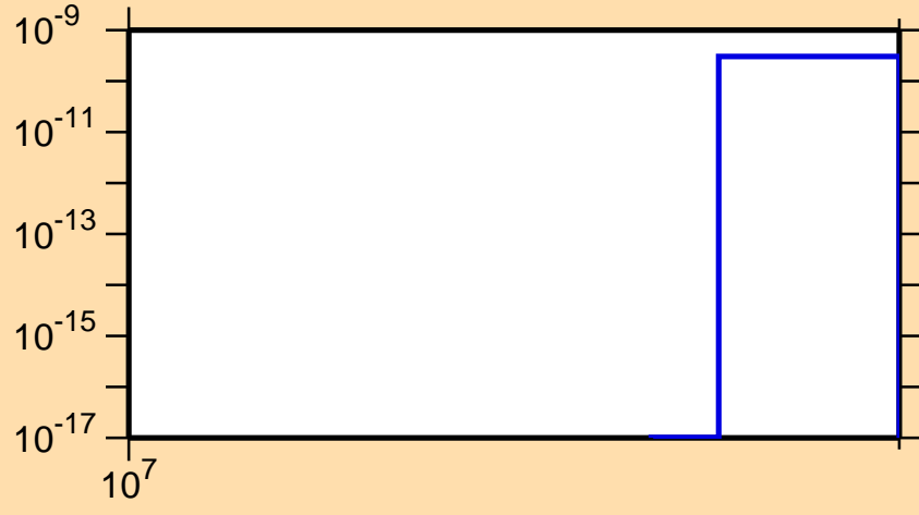
\sigma vs. E for ^{162}\text{Gd}(n,2np)
