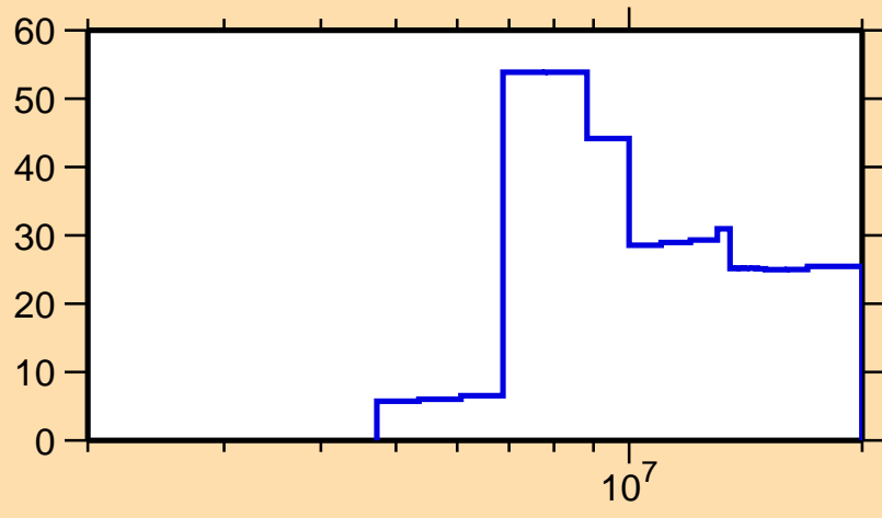
\Delta\sigma/\sigma vs. E for ^{162}\text{Gd}(n,n\text{cont.})
