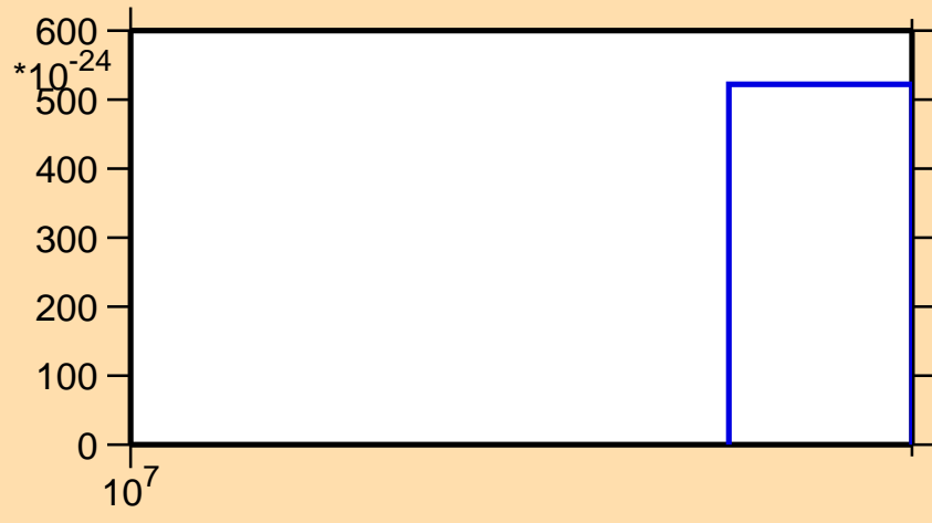
\sigma vs. E for ^{162}\text{Gd}(\text{mt } 11)
