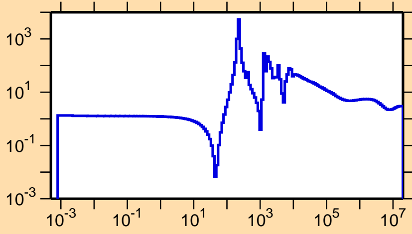
\sigma vs. E for ^{162}\text{Gd}(n,\text{el.})
