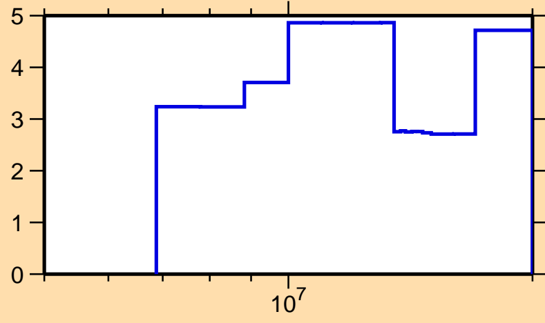
\Delta\sigma/\sigma vs. E for ^{162}\text{Gd}(n,\text{el.})
