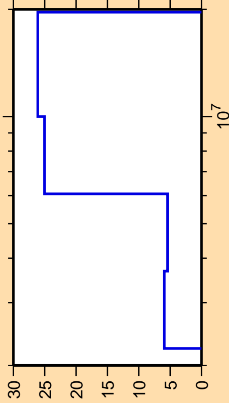
\Delta\sigma/\sigma vs. E for ^{162}\text{Gd}(n,\text{ncont.})
