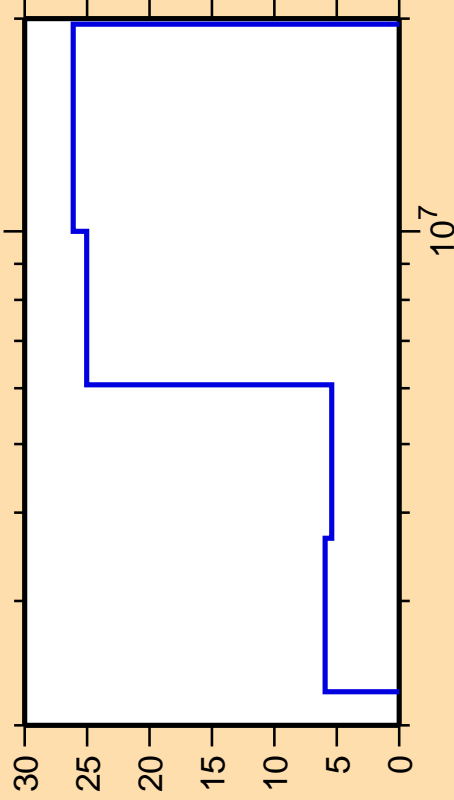
\Delta\sigma/\sigma vs. E for ^{162}\text{Gd}(n,n_{\text{cont}}) .
