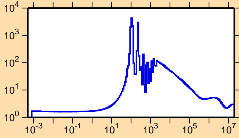
\sigma vs. E for ^{163}\text{Gd}(n,\text{el.})
