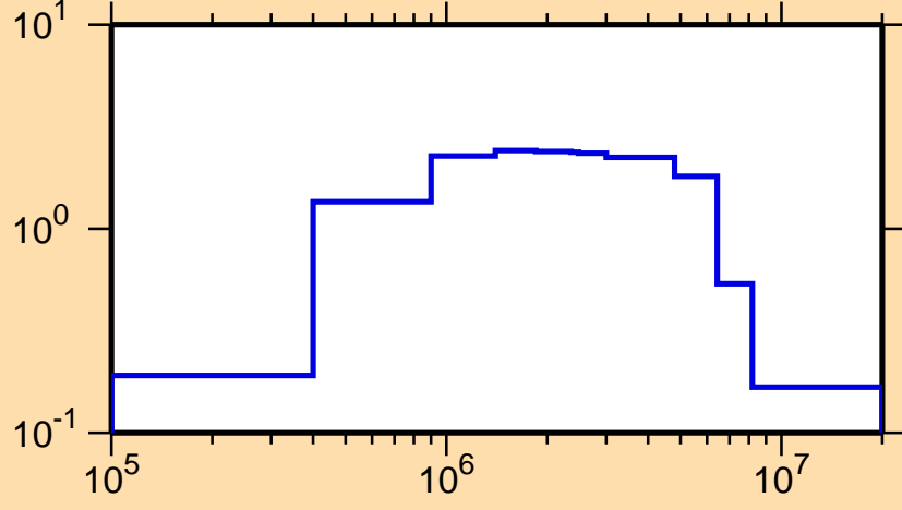
\sigma vs. E for ^{163}\text{Gd}(n,n\text{cont.})
