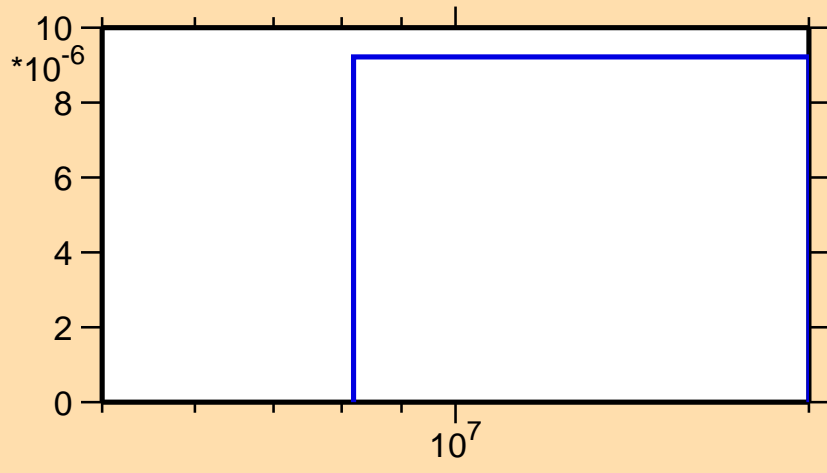
\sigma vs. E for ^{163}\text{Gd}(n,t)
