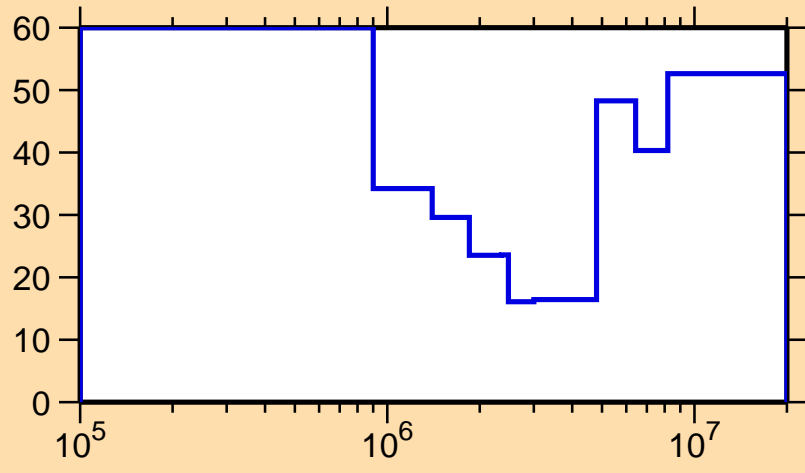
\Delta\sigma/\sigma vs. E for ^{163}\text{Gd}(n,n\text{cont.})
