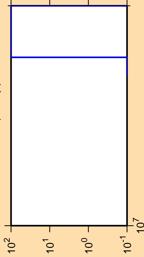
\Delta\sigma/\sigma vs. E for ^{164}\text{Gd}(n,2np)
