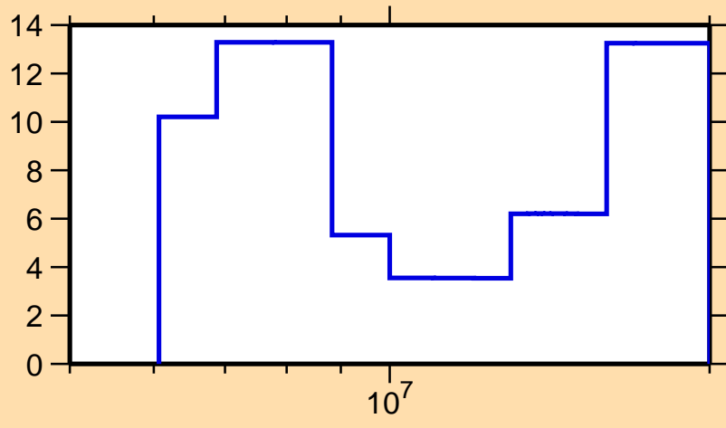
\Delta\sigma/\sigma vs. E for ^{164}\text{Gd}(n,\text{tot.})
