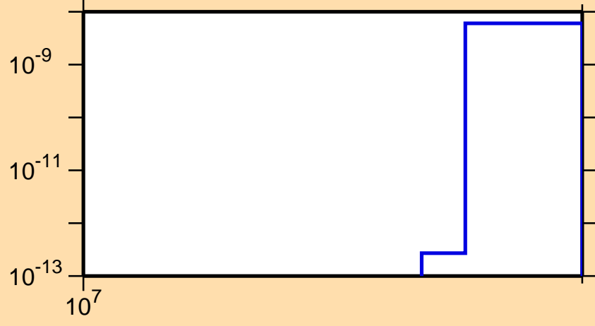
\sigma vs. E for ^{164}\text{Gd}(n,\text{nd})
