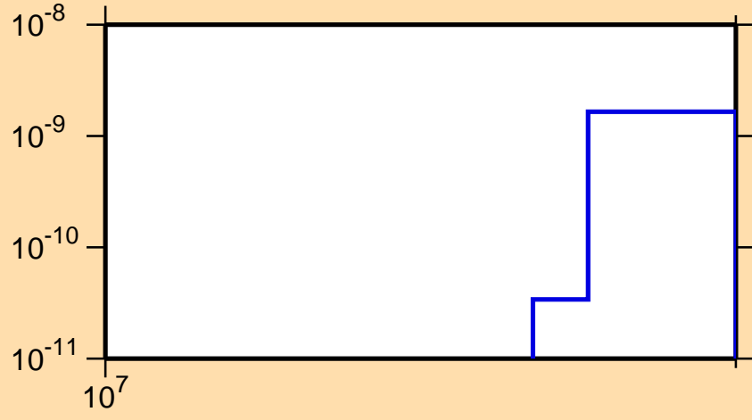
\sigma vs. E for ^{164}\text{Gd}(n,2n\alpha)
