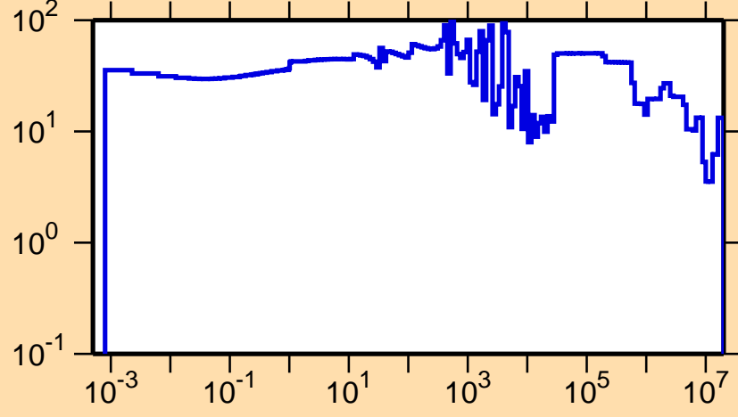
\Delta\sigma/\sigma vs. E for ^{164}\text{Gd}(n,\text{tot.})
