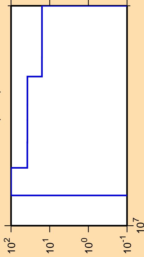
\Delta\sigma/\sigma vs. E for ^{164}\text{Gd}(n,3n)
