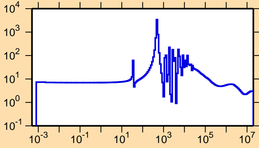
\sigma vs. E for ^{164}\text{Gd}(n,\text{el.})
