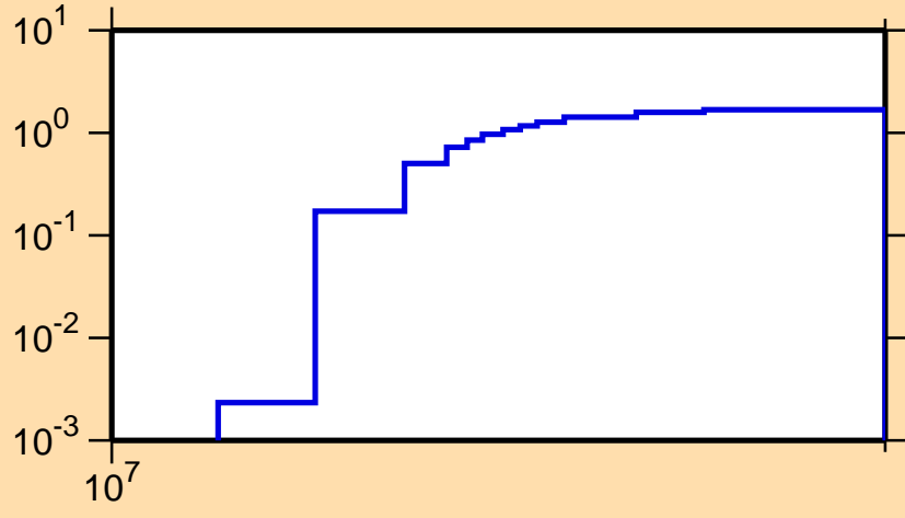
\sigma vs. E for ^{164}\text{Gd}(n,3n)
