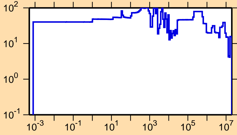
\Delta\sigma/\sigma vs. E for ^{164}\text{Gd}(n,\text{el.})
