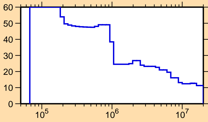
\Delta\sigma/\sigma vs. E for ^{164}\text{Gd}(n,\text{nonel.})
