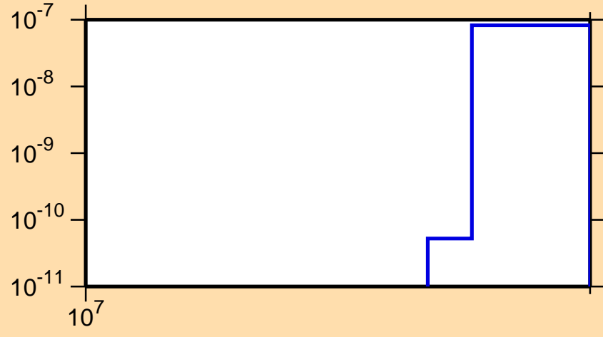
\sigma vs. E for ^{164}\text{Gd}(n,nt)
