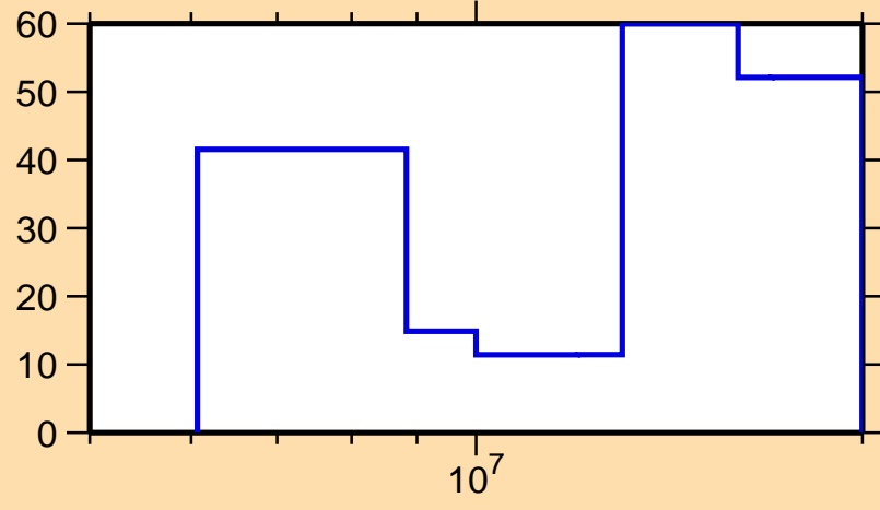
\Delta\sigma/\sigma vs. E for ^{164}\text{Gd}(n,2n)
