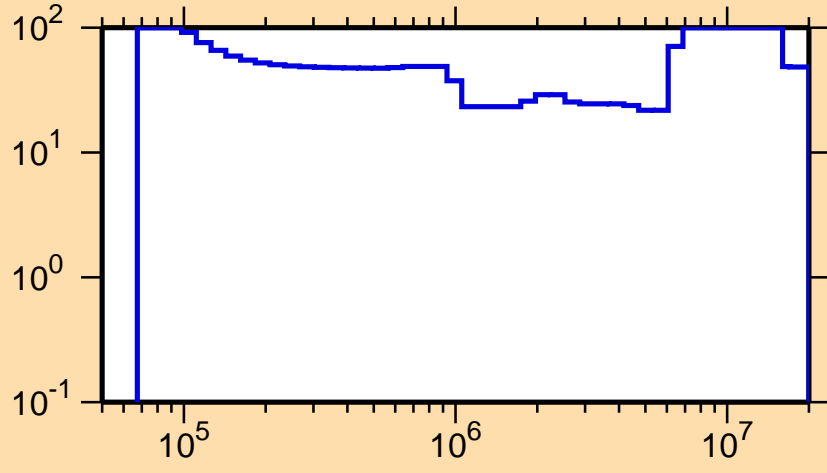
\Delta\sigma/\sigma vs. E for ^{164}\text{Gd}(n,\text{inel.})
