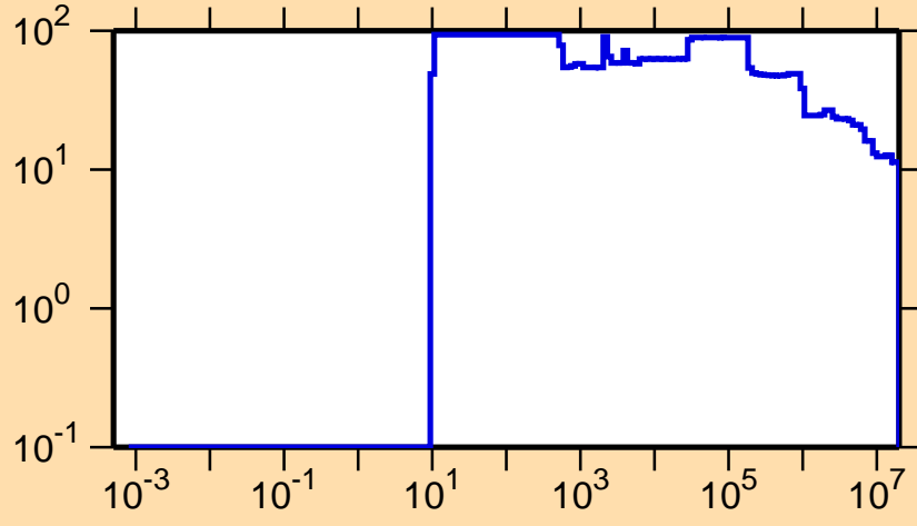
\Delta\sigma/\sigma vs. E for ^{164}\text{Gd}(n,\text{nonel.})
