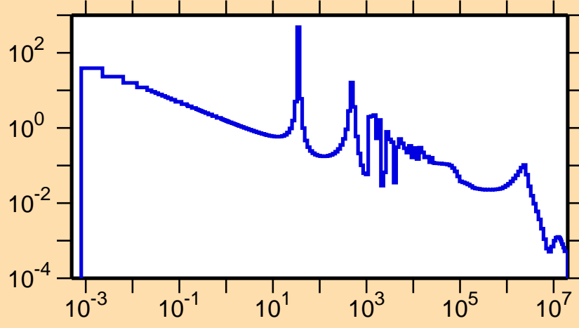
\sigma vs. E for ^{164}\text{Gd}(n,\gamma)
