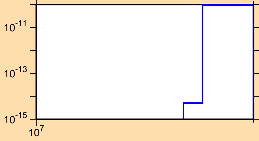
\sigma vs. E for ^{164}\text{Gd}(n,2np)
