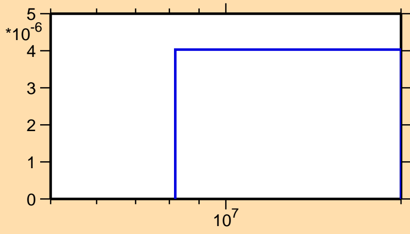
\sigma vs. E for ^{164}\text{Gd}(n,t)
