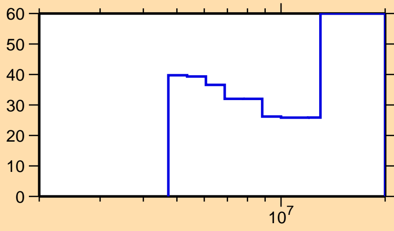
\Delta\sigma/\sigma vs. E for ^{165}\text{Gd}(n,2n)
