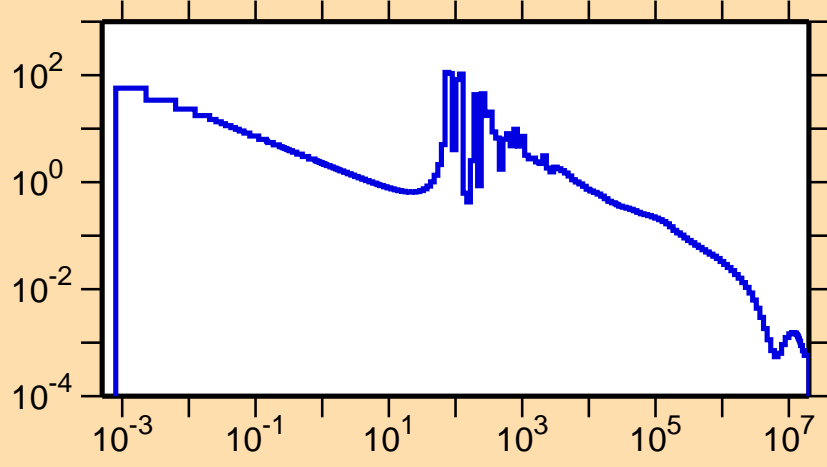
\sigma vs. E for ^{165}\text{Gd}(n,\gamma)
