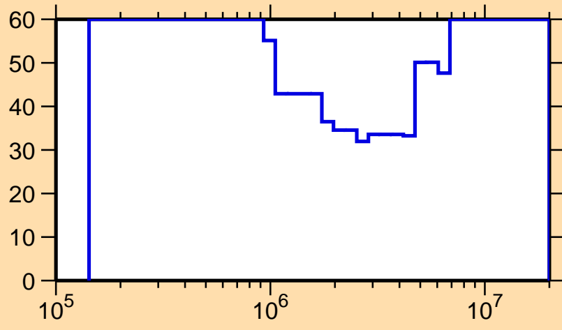
\Delta\sigma/\sigma vs. E for ^{165}\text{Gd}(n,\text{inel.})
