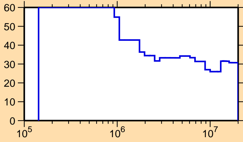
\Delta\sigma/\sigma vs. E for ^{165}\text{Gd}(n,\text{nonel.})
