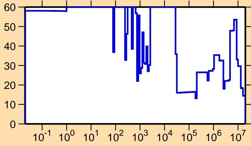
\Delta\sigma/\sigma vs. E for ^{165}\text{Gd}(n,\text{el.})
