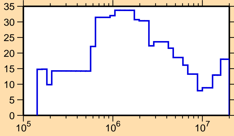
\Delta\sigma/\sigma vs. E for ^{165}\text{Gd}(n,\text{tot.})
