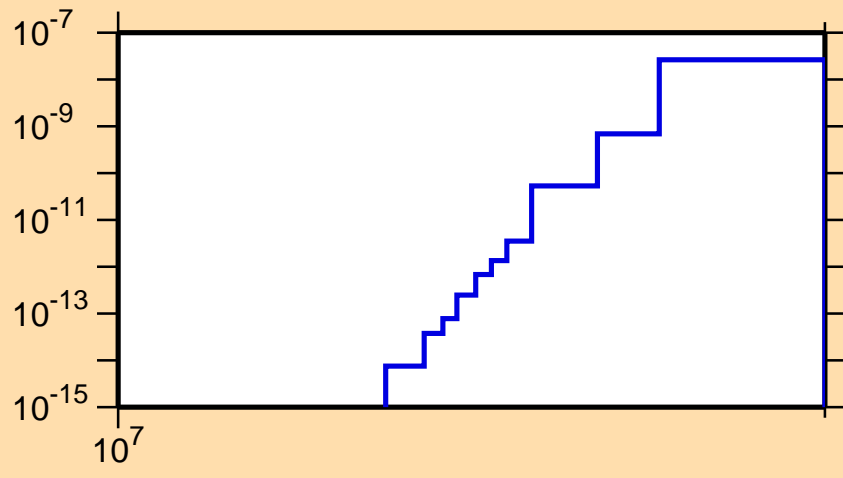
\sigma vs. E for ^{165}\text{Gd}(n,2n\alpha)
