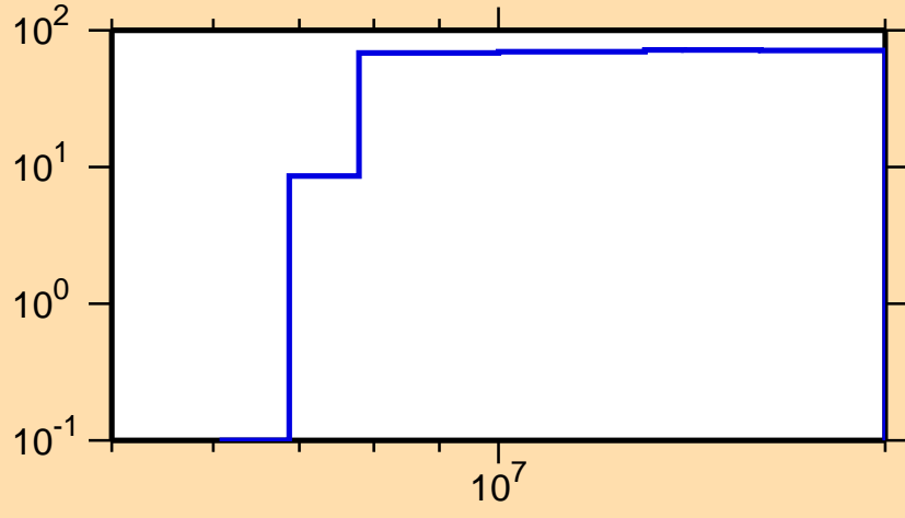
\Delta\sigma/\sigma vs. E for ^{165}\text{Gd}(n,p)
