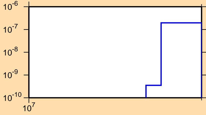
\sigma vs. E for ^{165}\text{Gd}(n,nt)
