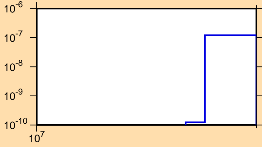
\sigma vs. E for ^{165}\text{Gd}(n,\text{nd})
