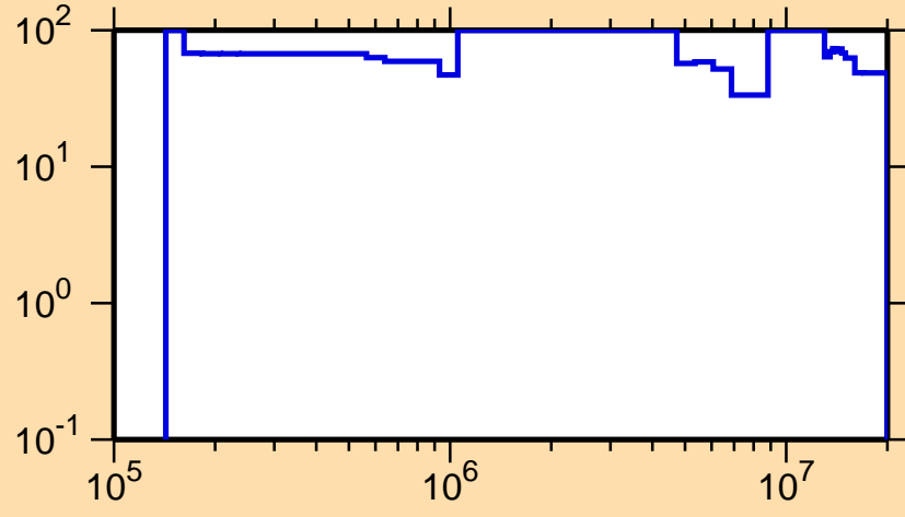
\Delta\sigma/\sigma vs. E for ^{165}\text{Gd}(n,n_1)
