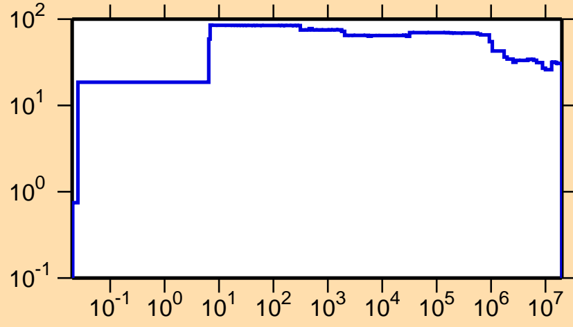
\Delta\sigma/\sigma vs. E for ^{165}\text{Gd}(n,\text{nonel.})
