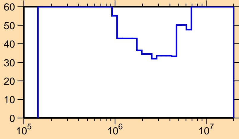
\Delta\sigma/\sigma vs. E for ^{165}\text{Gd}(n,\text{inel.})
