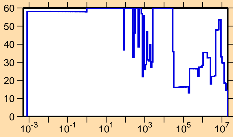
\Delta\sigma/\sigma vs. E for ^{165}\text{Gd}(n,\text{el.})
