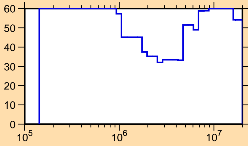
\Delta\sigma/\sigma vs. E for ^{165}\text{Gd}(n,n\text{cont.})
