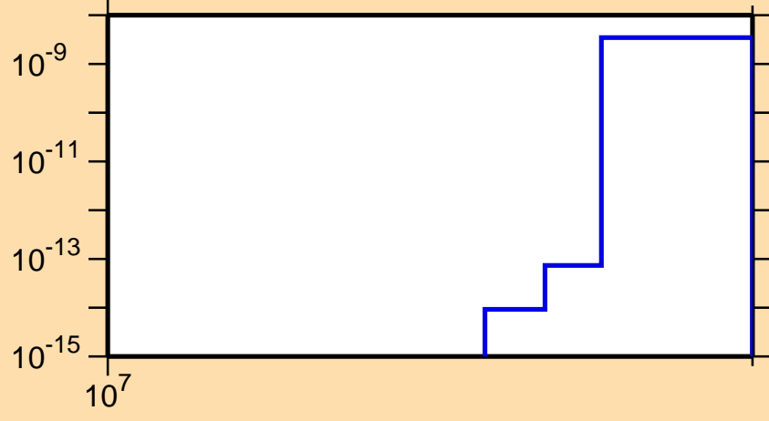
\sigma vs. E for ^{165}\text{Gd}(n,2np)
