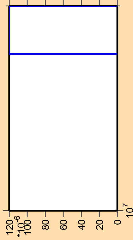
\Delta\sigma/\sigma vs. E for ^{165}\text{Gd} (mt 11)
