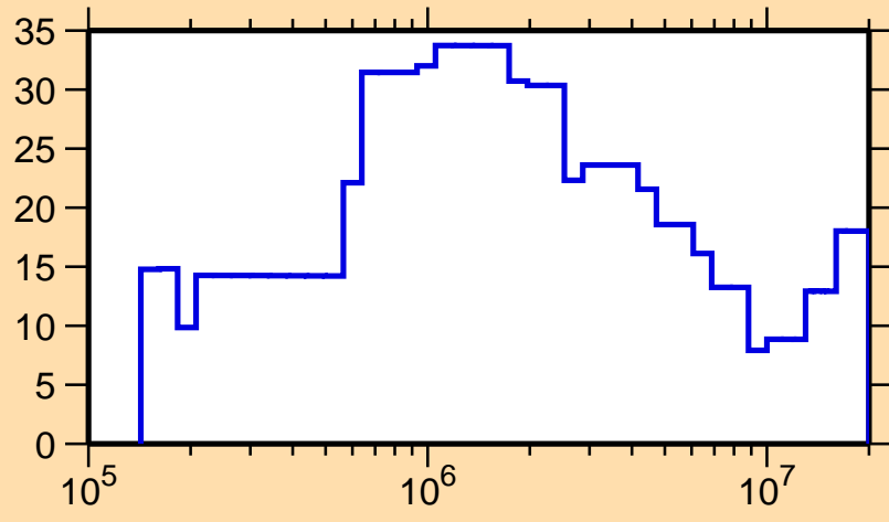
\Delta\sigma/\sigma vs. E for ^{165}\text{Gd}(n,\text{tot.})
