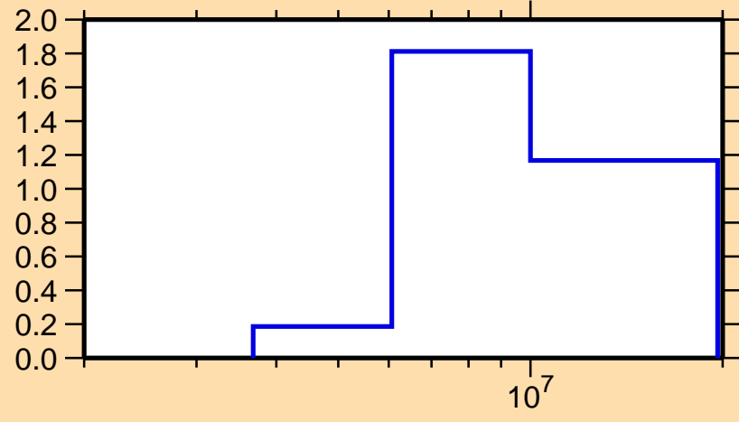
\sigma vs. E for ^{165}\text{Gd}(n,2n)
