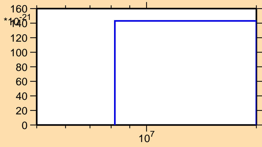
\sigma vs. E for ^{165}\text{Gd}(\text{mt } 11)
