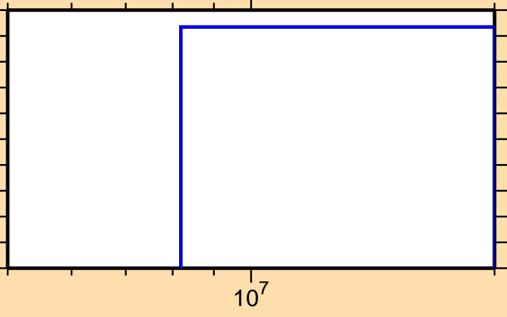
\sigma vs. E for ^{165}\text{Gd}(n,d)
