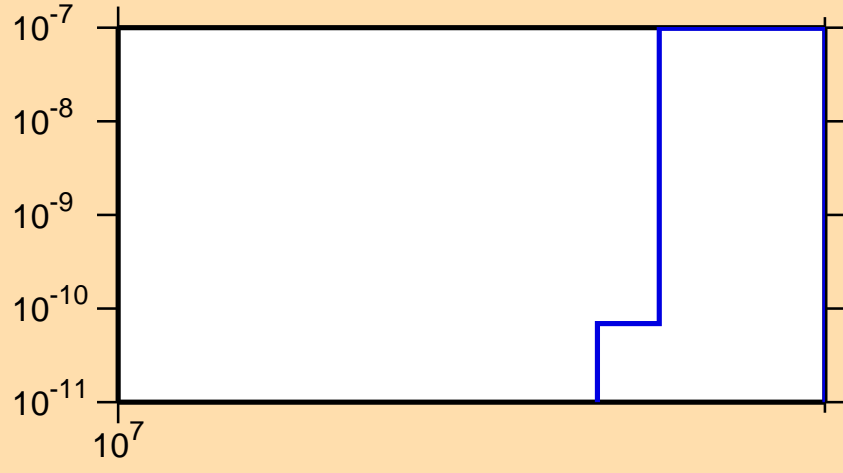
\sigma vs. E for ^{167}\text{Gd}(n,\text{nd})
