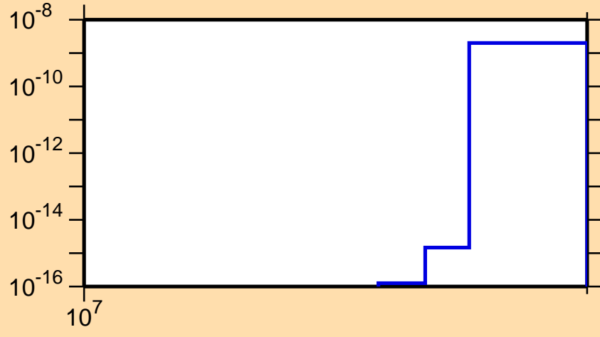
\sigma vs. E for ^{167}\text{Gd}(n,2np)
