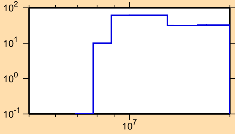
\Delta\sigma/\sigma vs. E for ^{167}\text{Gd}(n,p)
