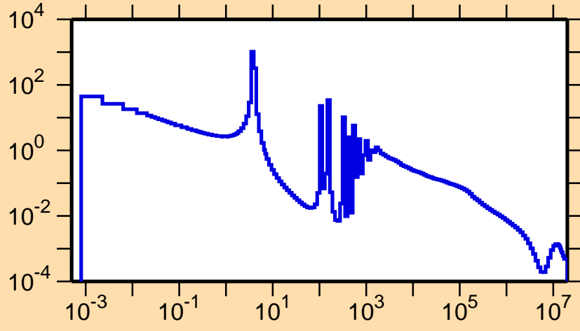
\sigma vs. E for ^{169}\text{Gd}(n,\gamma)
