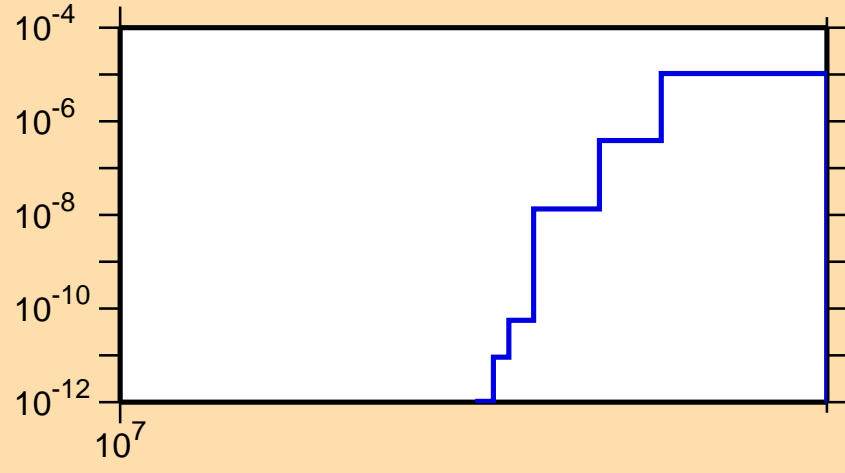
\sigma vs. E for ^{169}\text{Gd}(n,np)
