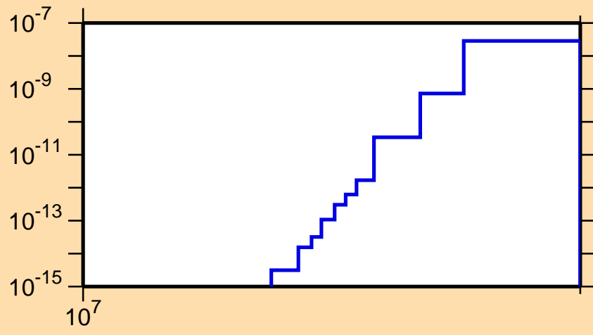
\sigma vs. E for ^{169}\text{Gd}(n,2n\alpha)
