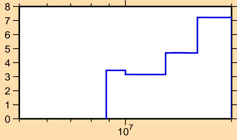
\Delta\sigma/\sigma vs. E for ^{169}\text{Gd}(n,\text{tot.})
