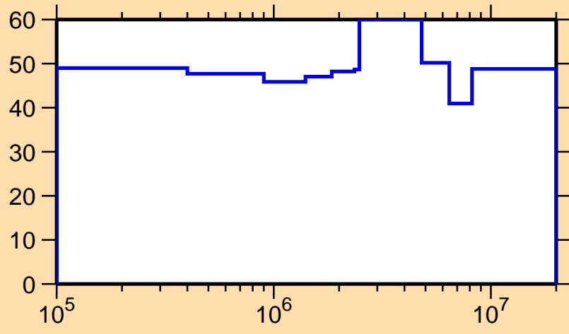
\Delta\sigma/\sigma vs. E for ^{169}\text{Gd}(n,n_1)
