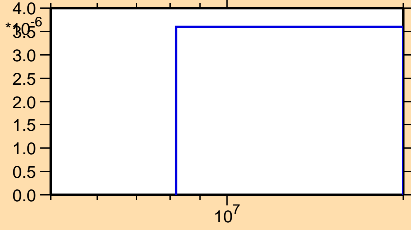
\sigma vs. E for ^{169}\text{Gd}(n,t)
