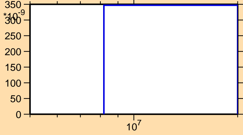
\sigma vs. E for ^{169}\text{Gd}(n,n\alpha)
