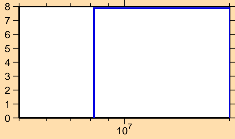
\Delta\sigma/\sigma vs. E for ^{169}\text{Gd}(n,\text{el.})
